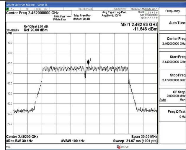
802.11n-HT20 Chain 1-High channel
