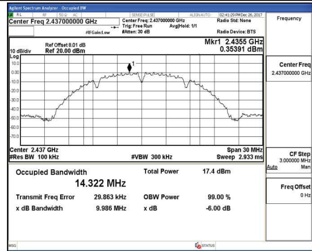
802.11b Chain 1-Middle channel
