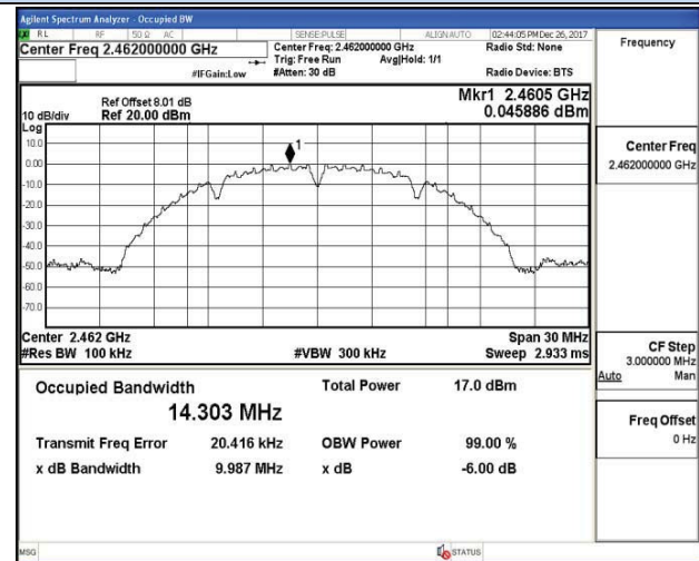
802.11b Chain 1-High channel
