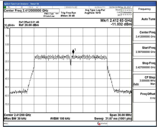
802.11n-HT20 Chain 1-Low channel
