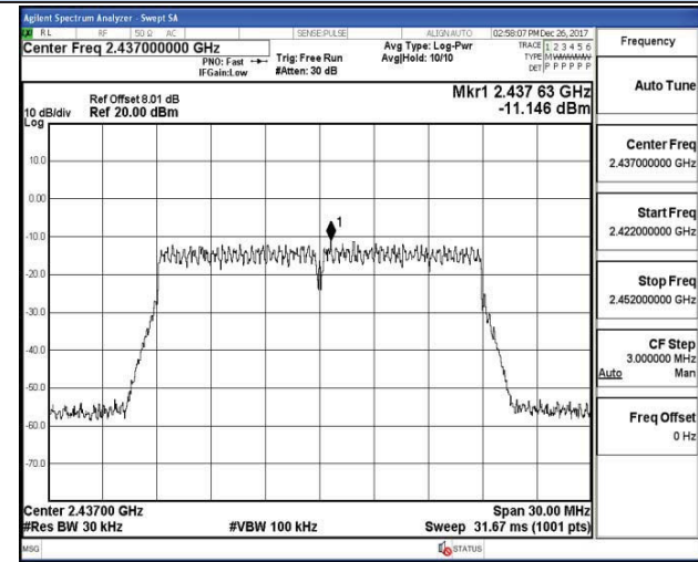
802.11n-HT20 Chain 1-Middle channel
