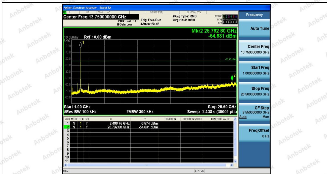
11N20_Ant1_2437_0~Reference
