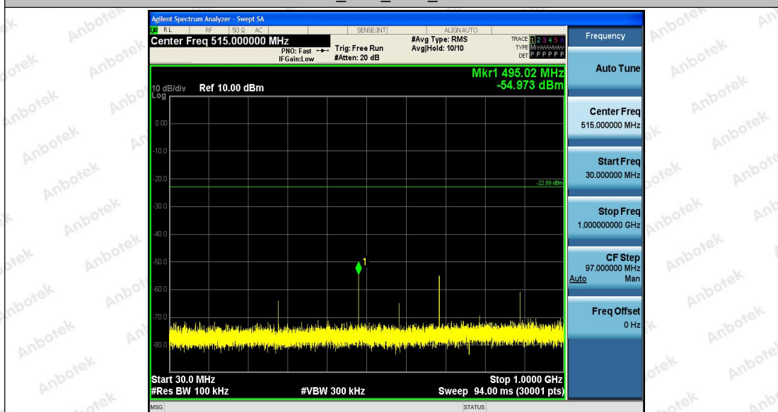
11N20_Ant1_2437_30~1000
