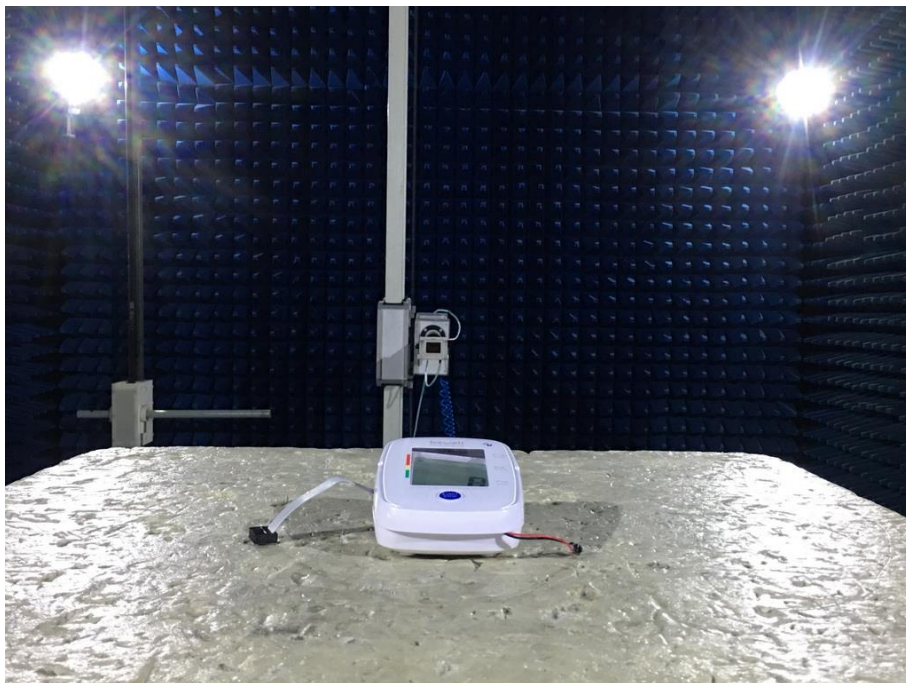
Photograph 6: Set-up for Radiated Spurious Emission, 18GHz - 26.5GHz
