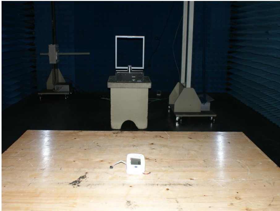
Photograph 3: Set-up for Radiated Spurious Emission, 9KHz - 30MHz
