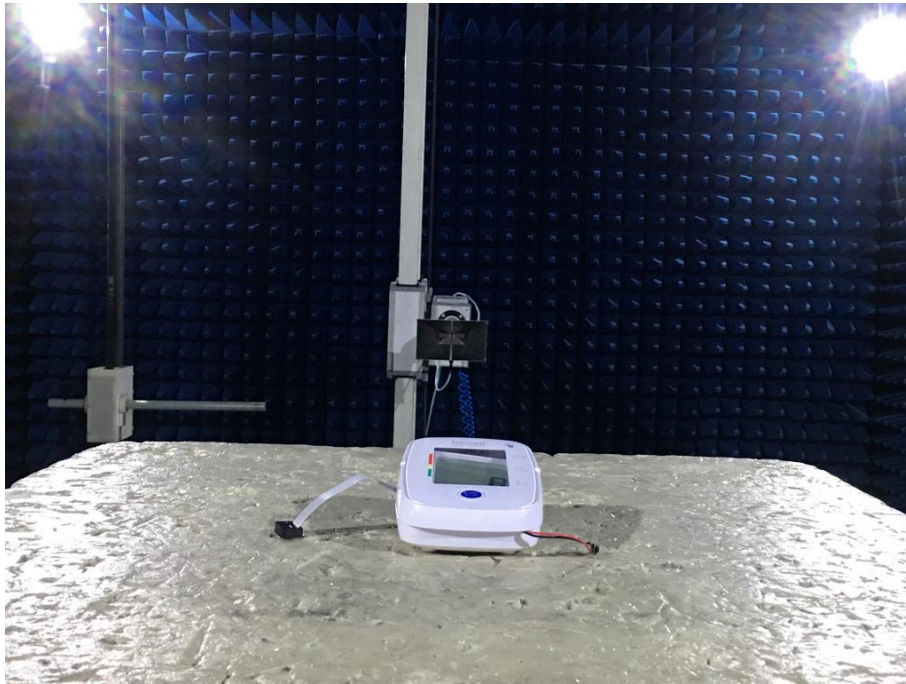
Photograph 5: Set-up for Radiated Spurious Emission, 1GHz - 18GHz
