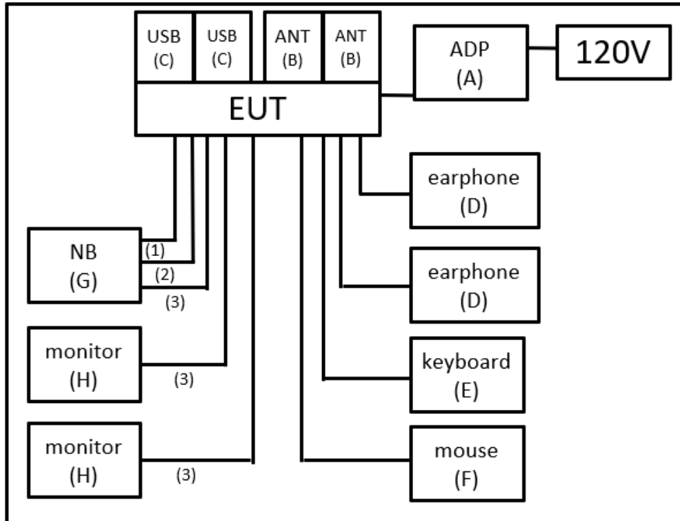
Radiated Emissions
