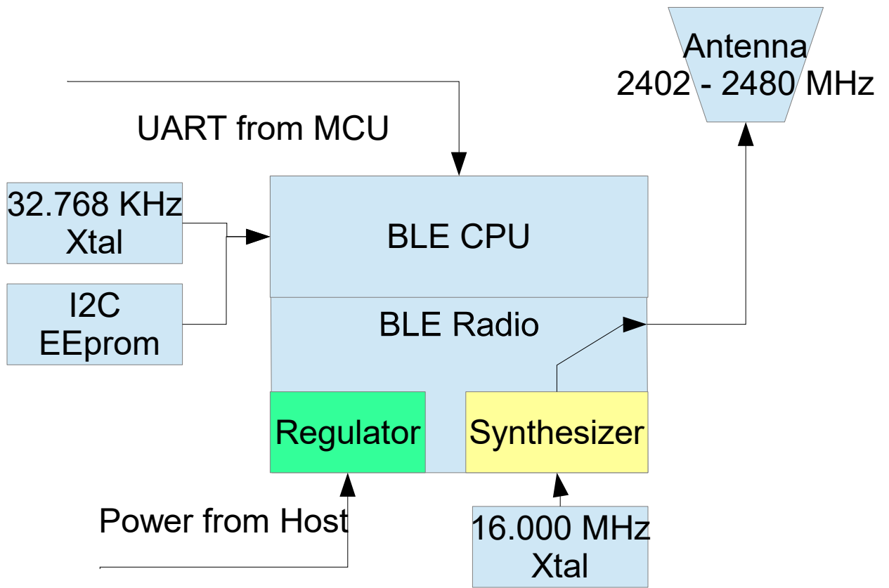
Frequency Block Diagram - Payrange BluKey Select
