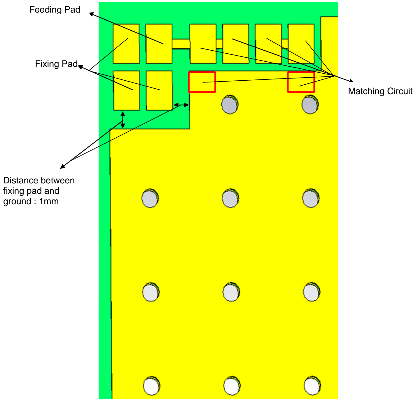
FIGURE 2: RECOMMENDED PCB LAYOUT
