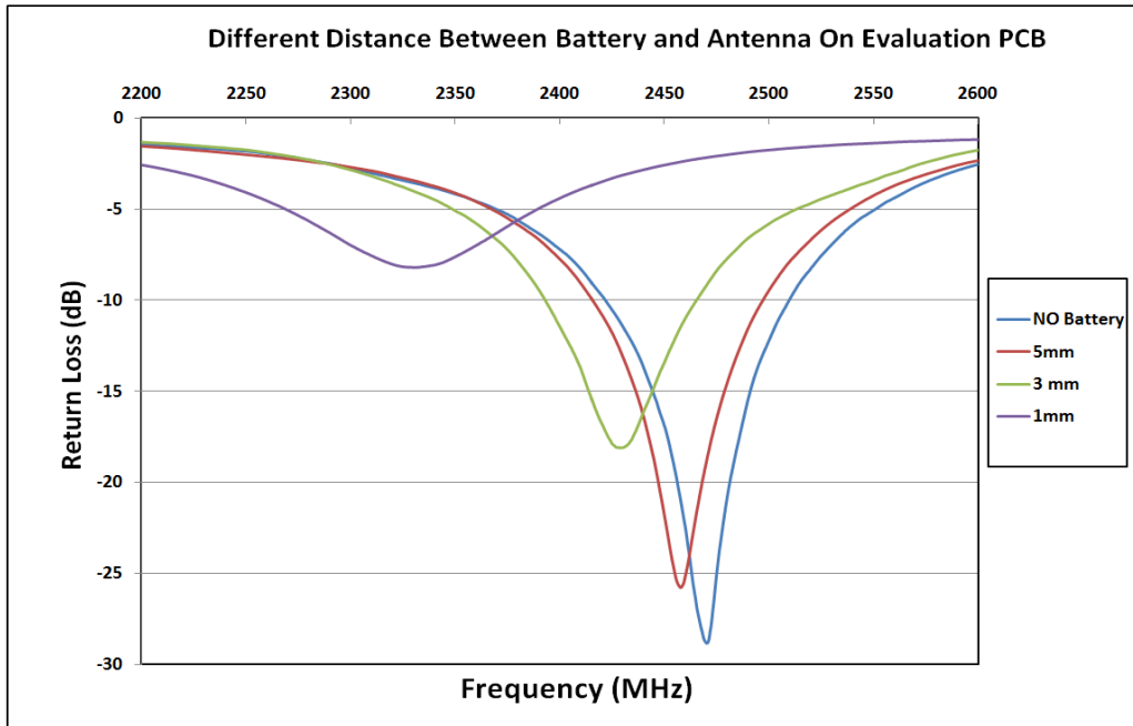
Figure 12: Return loss comparison of battery distance from antenna
