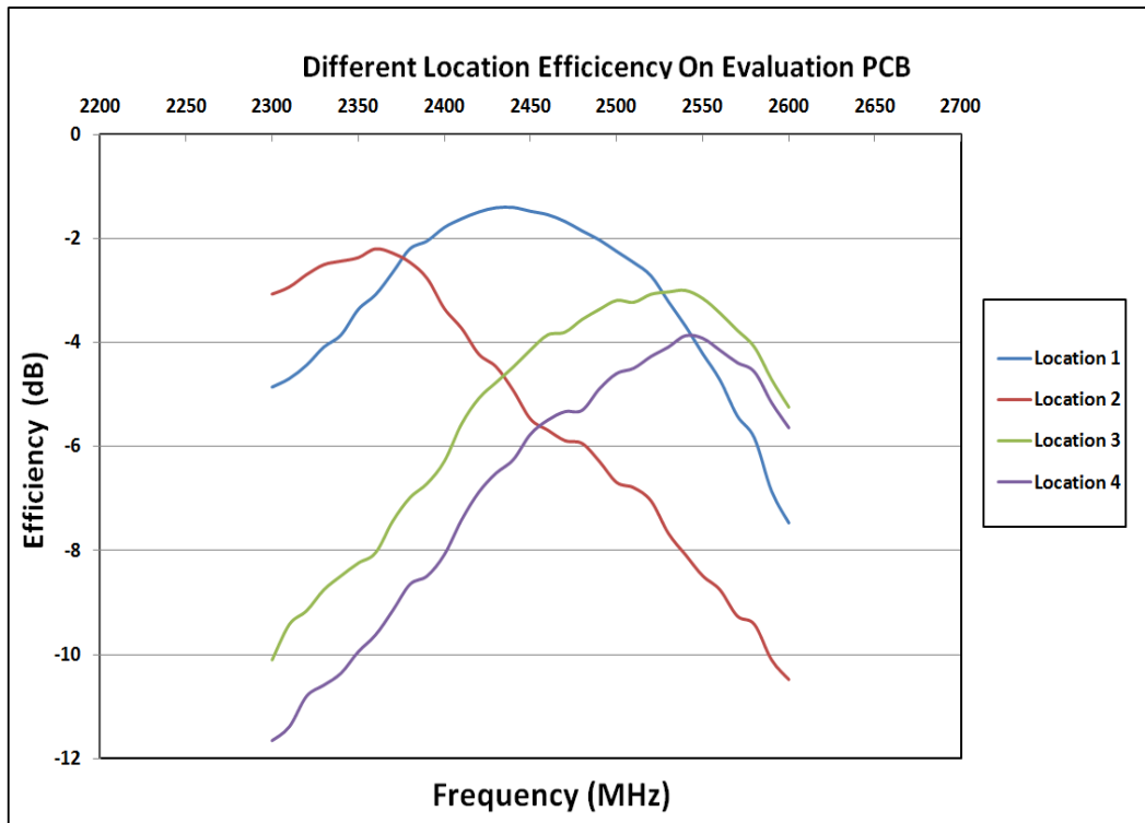
Figure 7: Total efficiency of comparison of different location on PCB
