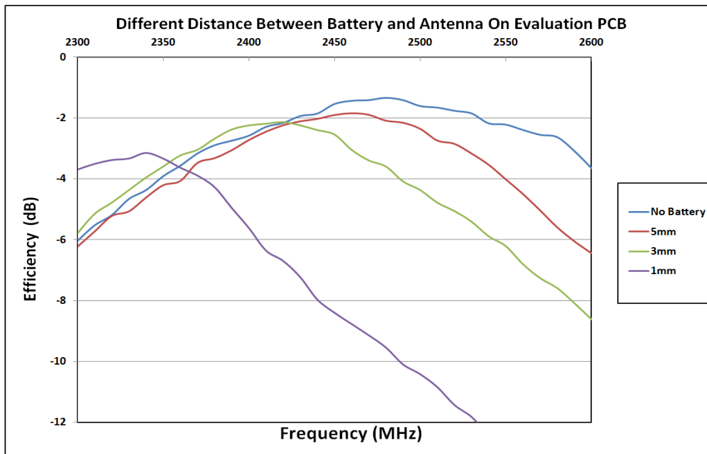
Figure 13: Total efficiency comparison of battery distance from antenna
