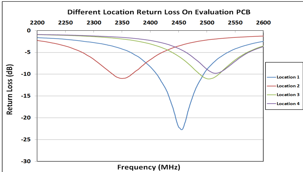
Figure 6: Return loss of comparison of different location on PCB
