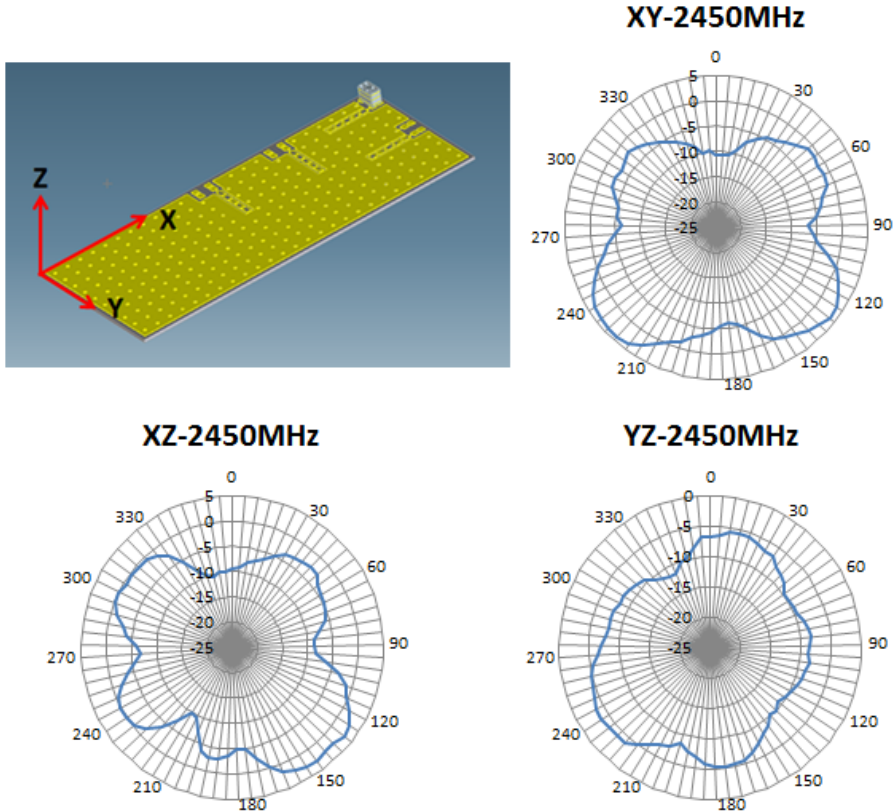
Figure 14: Radiation Pattern of antenna at 2.45GHz at Free space
