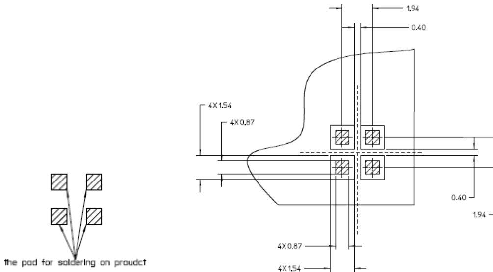
Figure 18: Footprint on PCB for soldering
