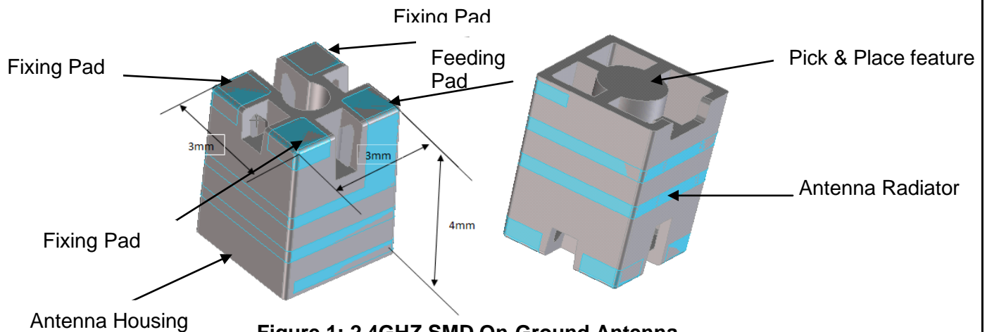
Figure 1: 2.4GHZ SMD On-Ground Antenna
