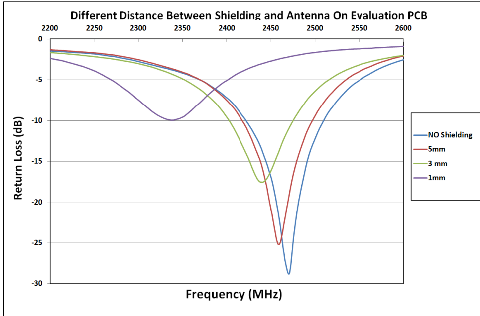
Figure 9: Return loss comparison of shielding can distance from antenna
