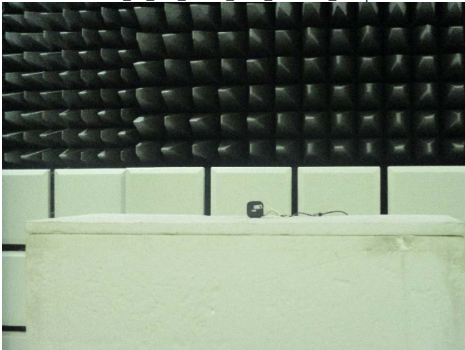
Part_15_247_WLAN_2.4G_Radiated_Setup
