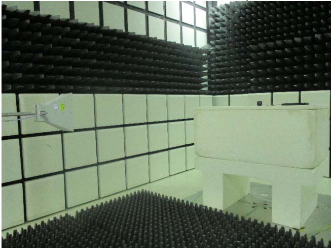
Part_15_247_OFDM_Radiated_Setup
