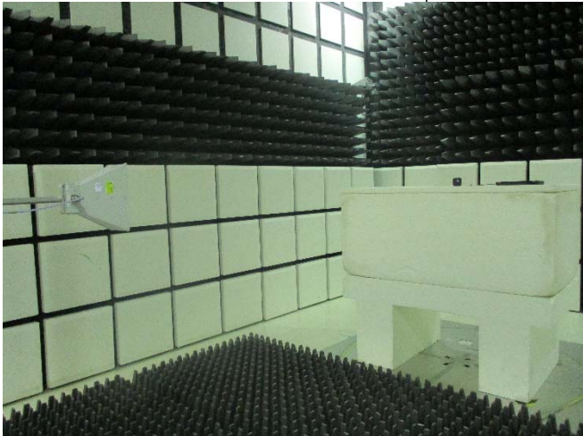
Part_15_247_FSK_Radiated_Setup
