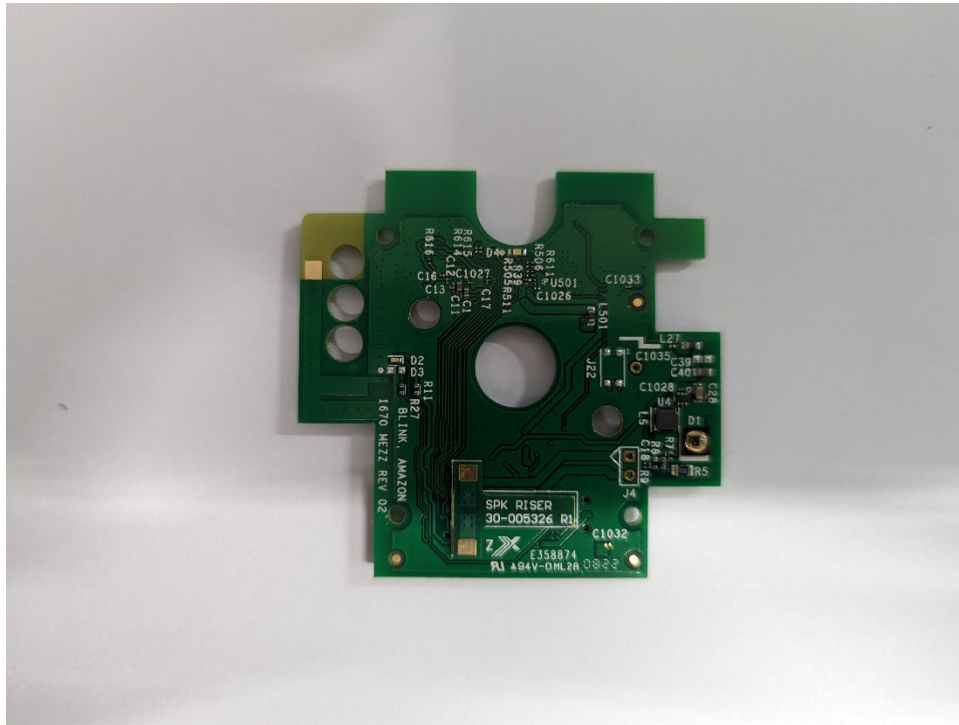
Mezz Board Side 1
