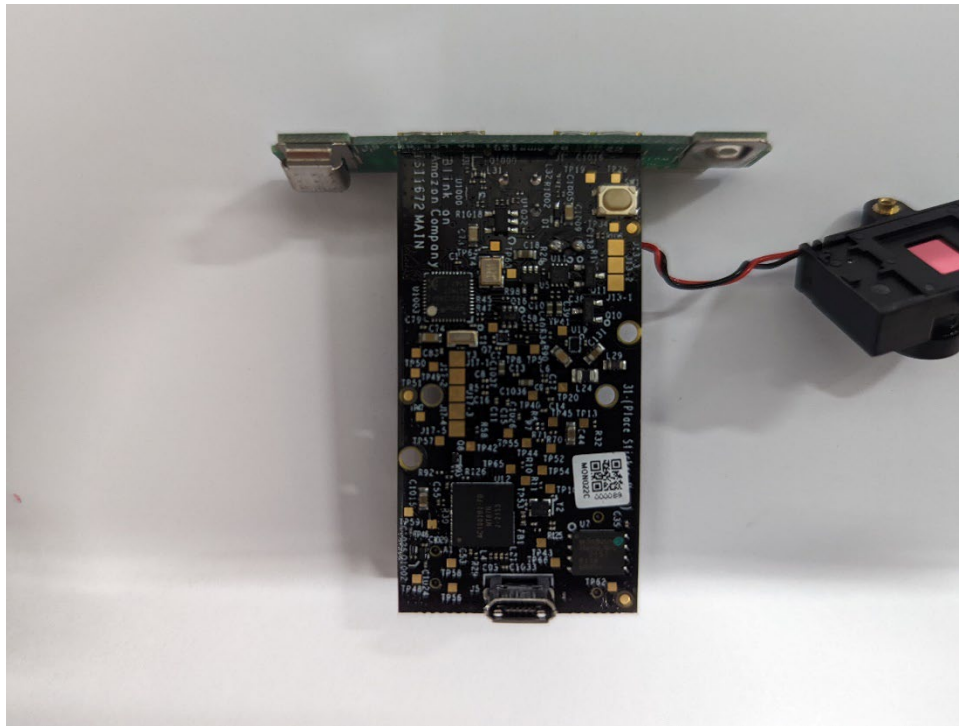
Main Board, Battery /LFR Antenna Board Attached, Side 2
