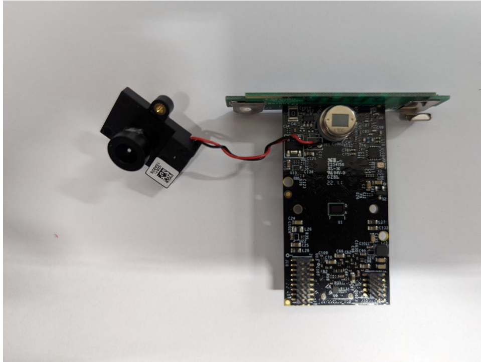
Main Board, Battery /LFR Antenna Board Attached, Side 1
