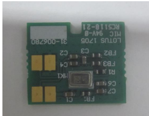
Mic Board Bottom Side
