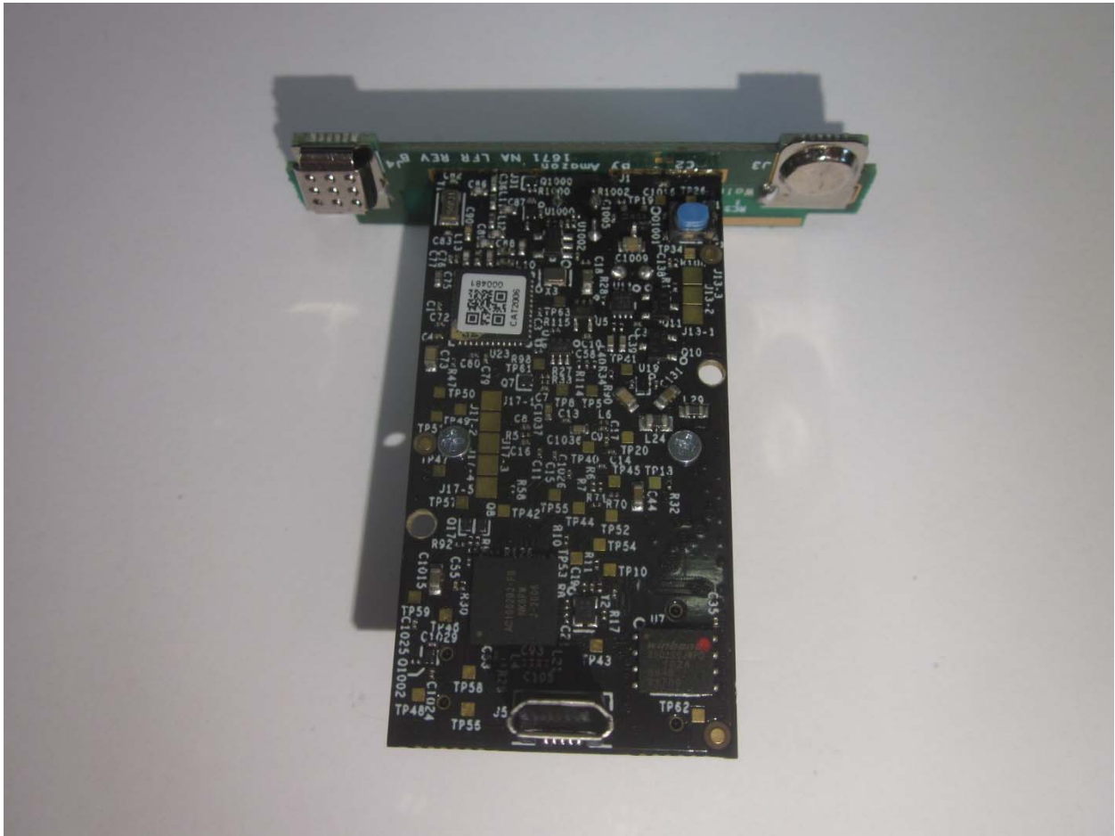
Main Board, Battery /LFR Antenna Board Attached, Side 1 Battery /LFR Antenna Board bottom
