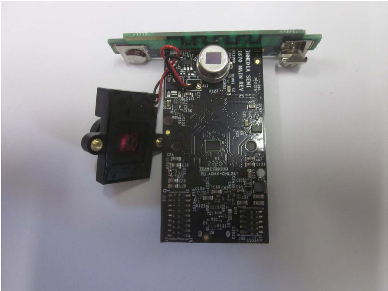
Main Board Camera shutter removed, Battery / LFR Antenna Board Attached, Side 2
