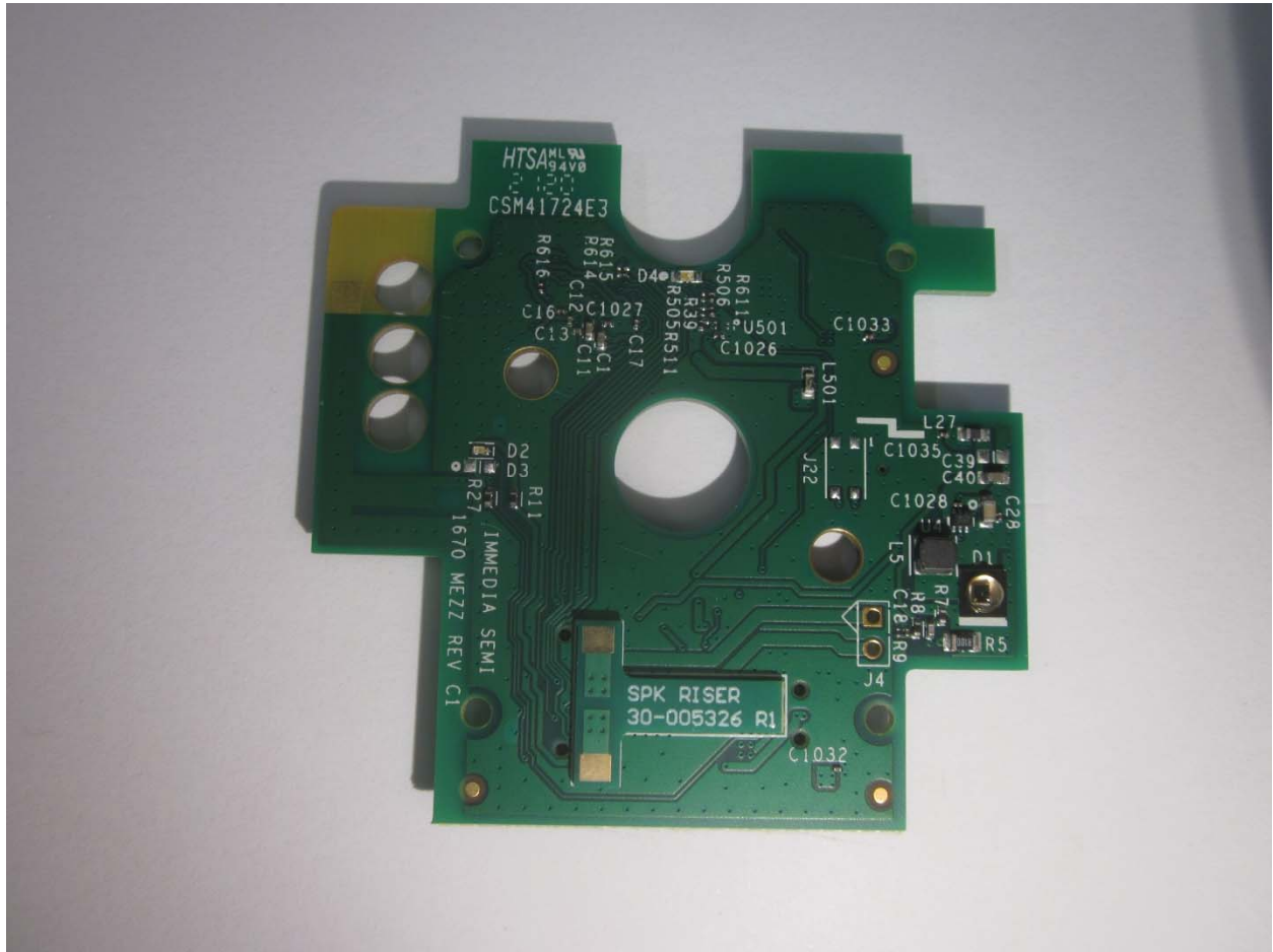
Mezz Board Side 1
