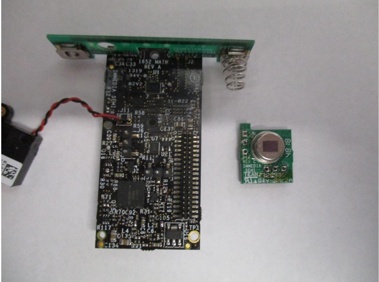
Main Board with Camera PIR Board Removed, Battery /Antenna Board Attached
