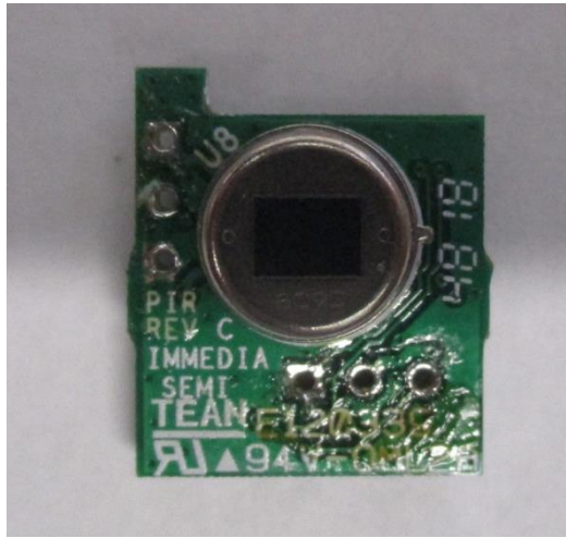
PIR Board Side1
