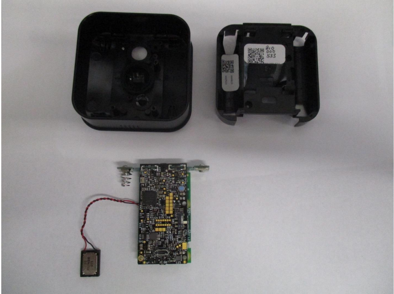
Electronics removed from enclosure
