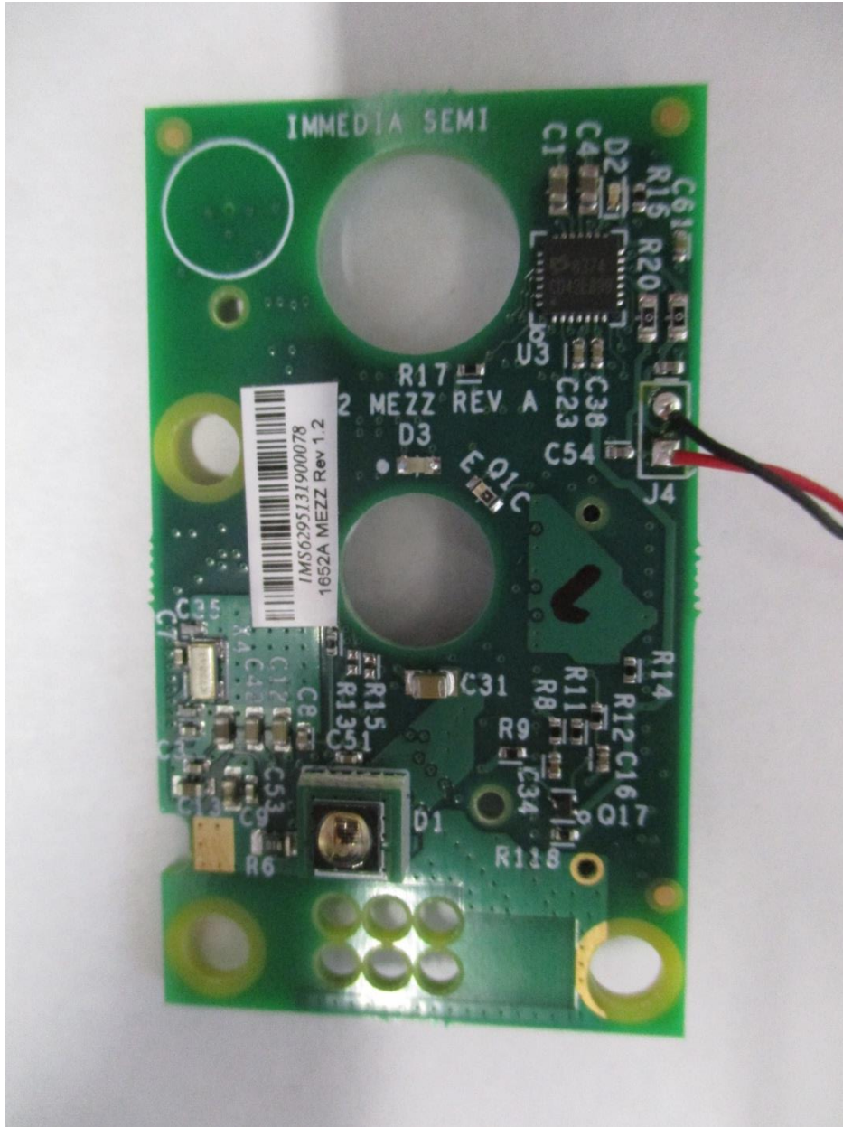
Mezz Board Side 2
