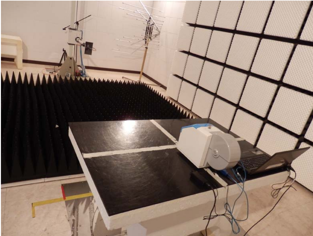
Photograph 3: Test Setup for Above 1 GHz
