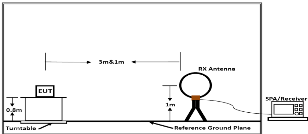
Below 30MHz
