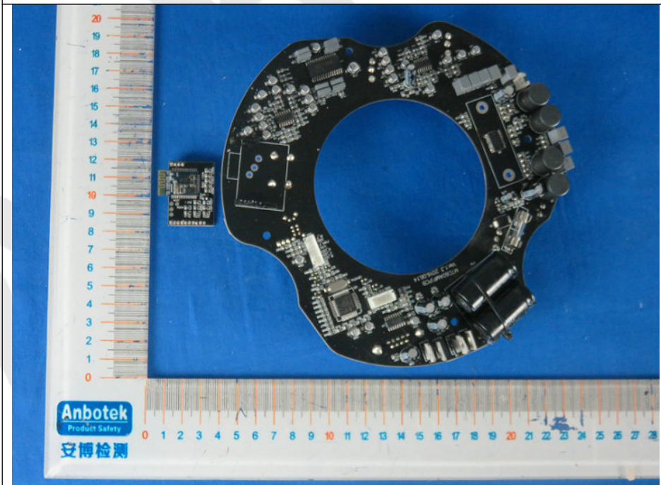
2. Figure PCB of the EUT-Front View
