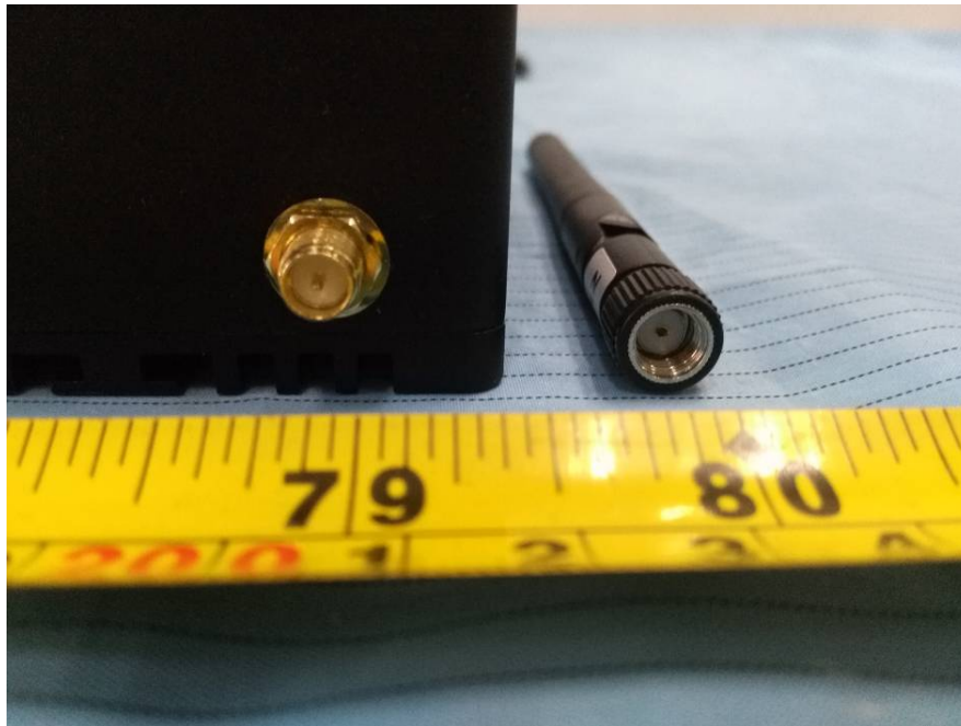
EUT – Lola Antenna Port View
