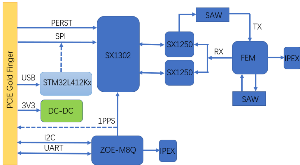
Figure 3 | RAK2287Block Diagram
