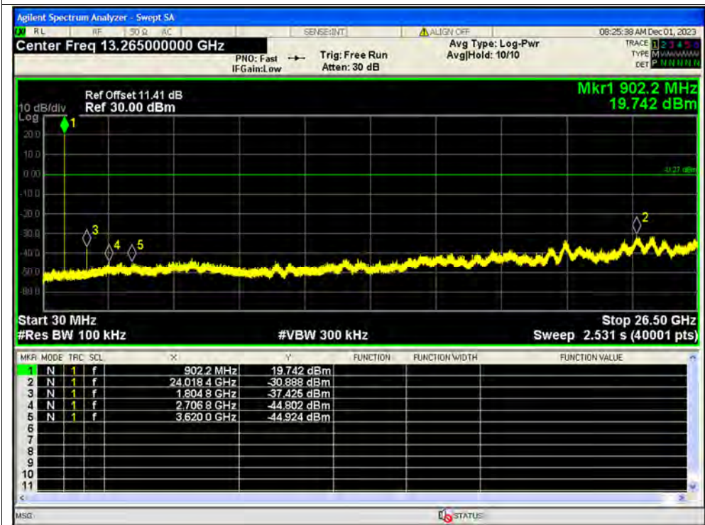
Tx. Spurious NVNT LoRa FHSS_SF7 902.3MHz Ant1 Emission
