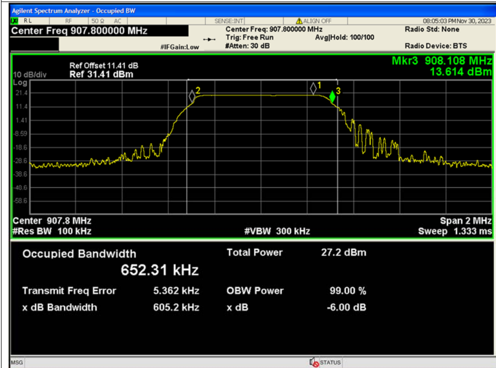
-6dB Bandwidth NVNT LoRa DTS_SF8 907.8MHz Ant1
