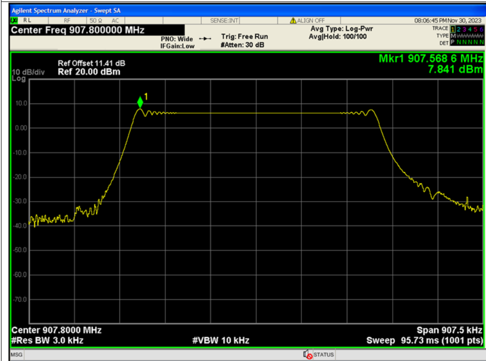
PSD NVNT LoRa DTS_SF8 907.8MHz Ant1
