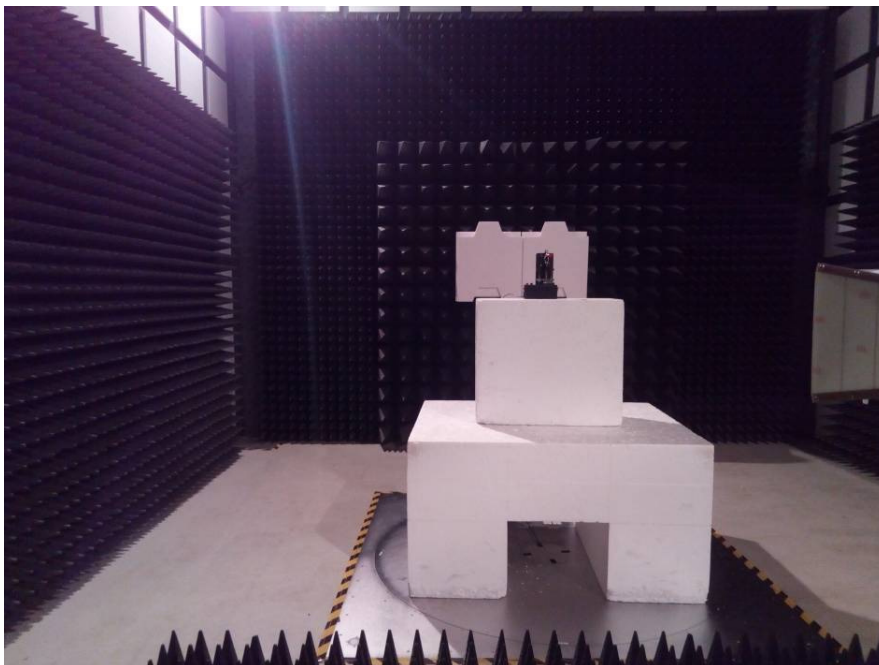
Radiated Emissions View (Above 1 GHz, Onboard Antenna)
