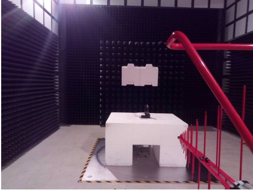
Radiated Emissions View (Below 1 GHz, External Antenna)
