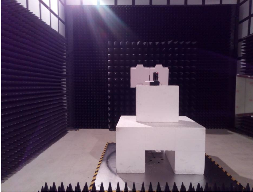
Radiated Emissions View (Above 1 GHz, External Antenna)
