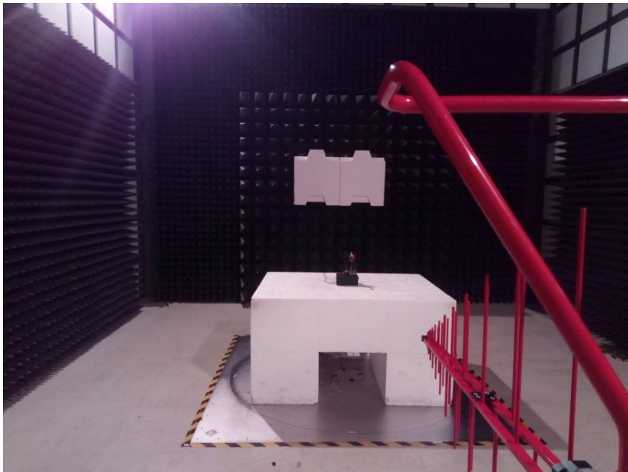
Radiated Emissions View (Below 1 GHz, Onboard Antenna)
