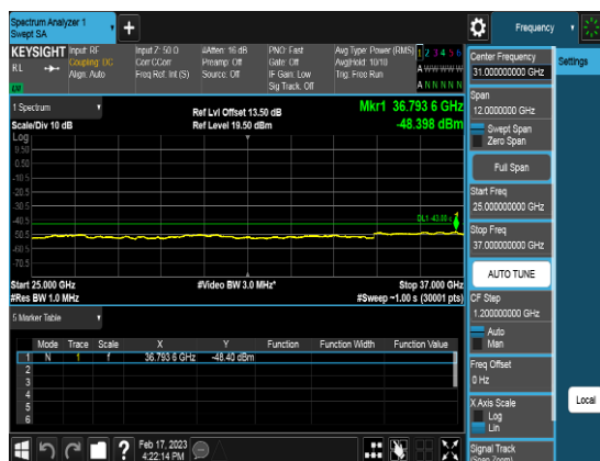
Port1_20M_3560.01MHz_TM3.1a_CHL_CSE3
