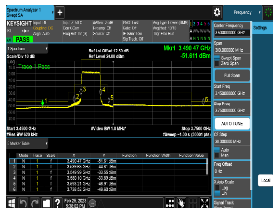
Port1_30M_3565.02MHz_TM3.1a_CHL_CSEpart 96
