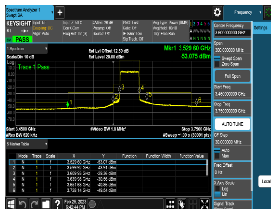
Port1_30M_3624.99MHz_TM3.1a_CHM_CSEpar 196
