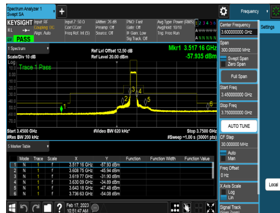
Port2_10M_3624.99MHz_TM3.1a_CHM_CSEpar 196
