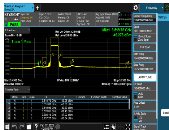
Port1_20M_3560.01MHz_TM3.1a_CHL_CSEpart 96
