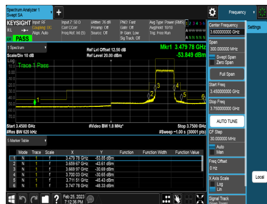
Port1_30M_3684.99MHz_TM3.1a_CHH_CSEpart 96
