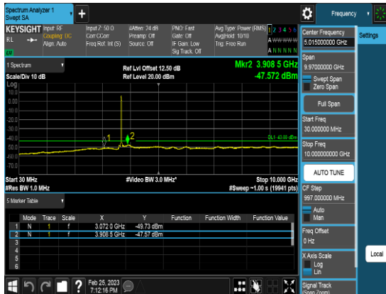
Port1_30M_3684.99MHz_TM3.1a_CHH_CSE3
