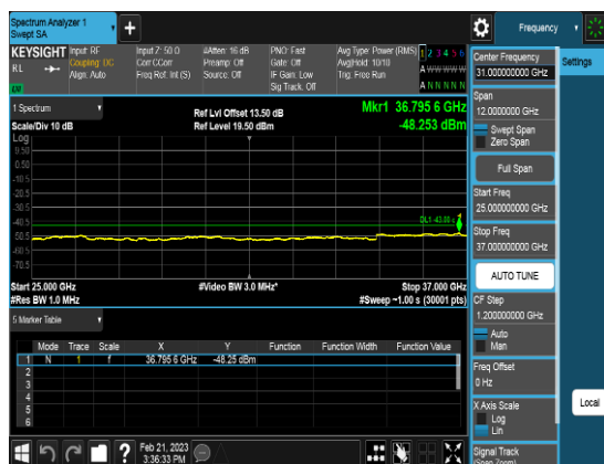
Port1_40M_3679.98MHz_TM3.1a_CHH_CSE3
