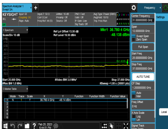
Port1_30M_3624.99MHz_TM3.1a_CHM_CSE3
