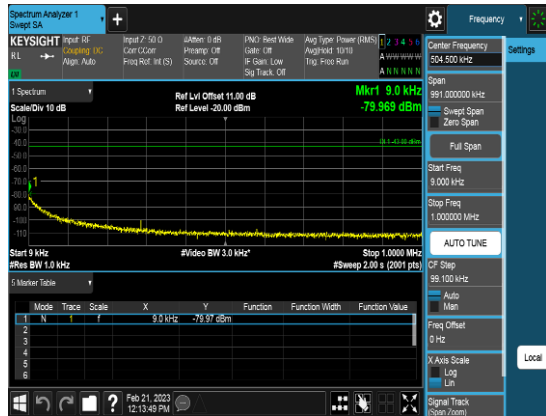
Port1_40M_3624.99MHz_TM3.1a_CHM_CSE1
