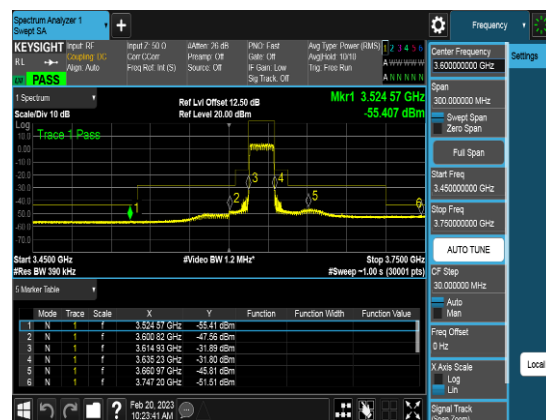
Port1_20M_3624.99MHz_TM3.1a_CHM_CSEpar 196
