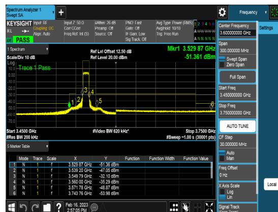
Port2_10M_3555MHz_TM3.1a_CHL_CSEpart98
