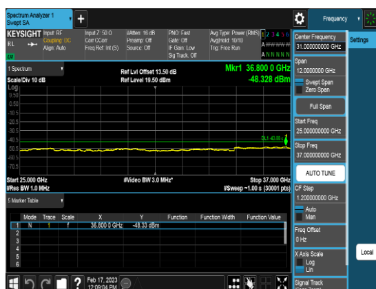
Port2_10M_3694.98MHz_TM3.1a_CHH_CSE3
