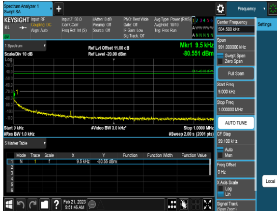
Port2_40M_3570MHz_TM3.1_CHL_CSE1
