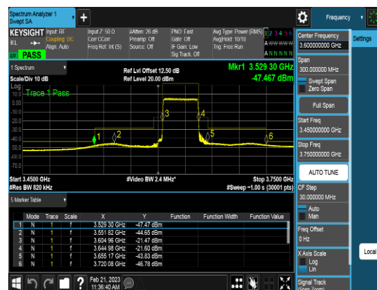
Port2_40M_3624.99MHz_TM3.1_CHM_CSEpart 96
