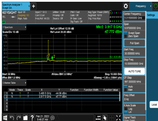
Port2_40M_3570MHz_TM3.1_CHL_CSE3
