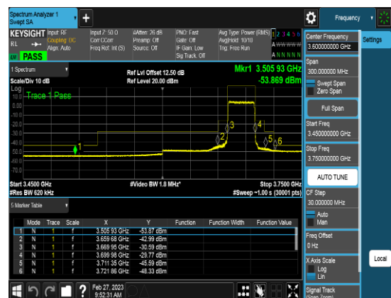
Port2_30M_3684.99MHz_TM3.1_CHH_CSEpart9 6
