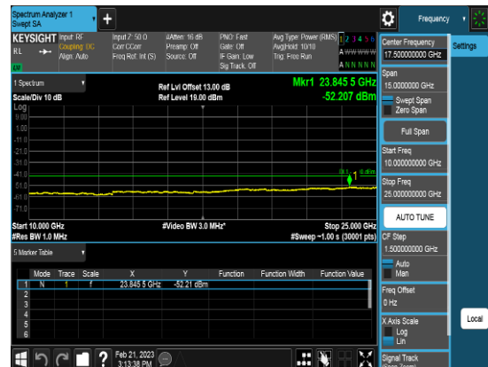
Port2_40M_3679.98MHz_TM3.1_CHH_CSEpart9 6
