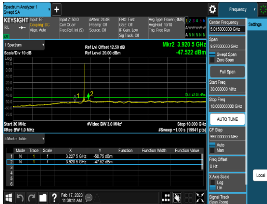
Port2_10M_3694.98MHz_TM3.1_CHH_CSE3
