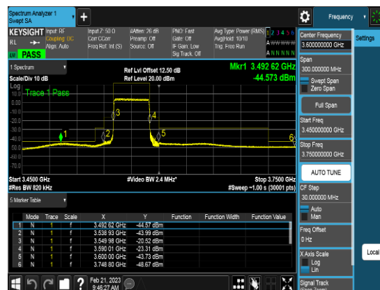
Port2_40M_3570MHz_TM3.1_CHL_CSEpart96
