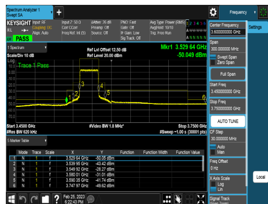
Port2_30M_3565.02MHz_TM3.1_CHL_CSEpart 6
