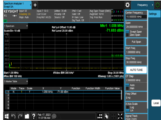
Port2_10M_3694.98MHz_TM3.1_CHH_CSE2
