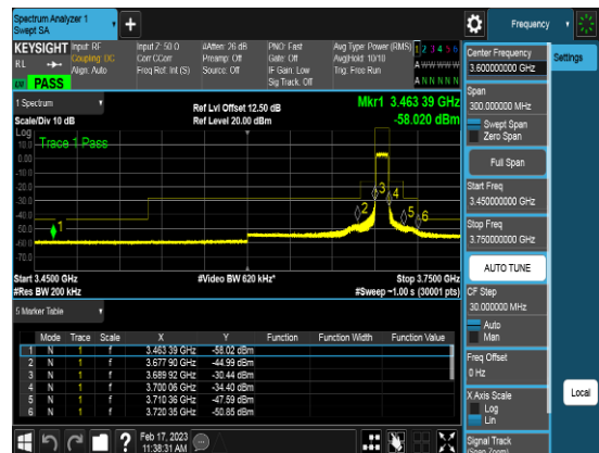
Port2_10M_3694.98MHz_TM3.1_CHH_CSEpart9 6
