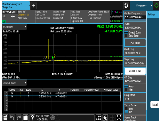
Port2_20M_3560.01MHz_TM3.1_CHL_CSE3
