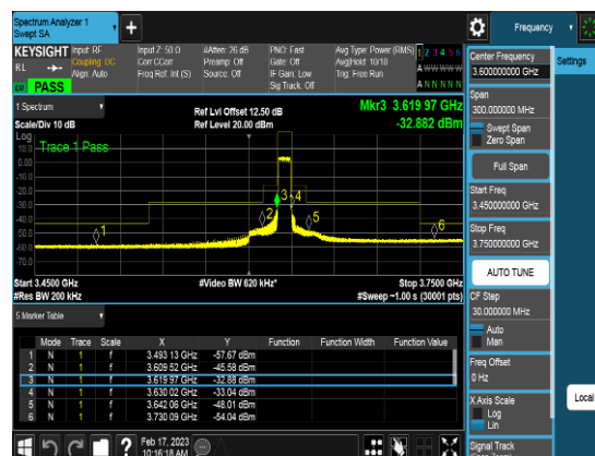
Port2_10M_3624.99MHz_TM3.1_CHM_CSEpart 96
