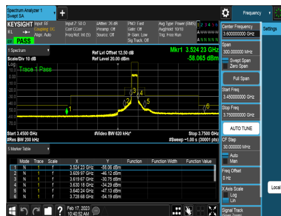
Port1_10M_3624.99MHz_TM3.1a_CHM_CSEpar 196
