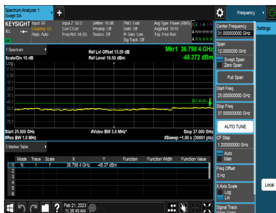
Port2_40M_3624.99MHz_TM3.1_CHM_CSE3
