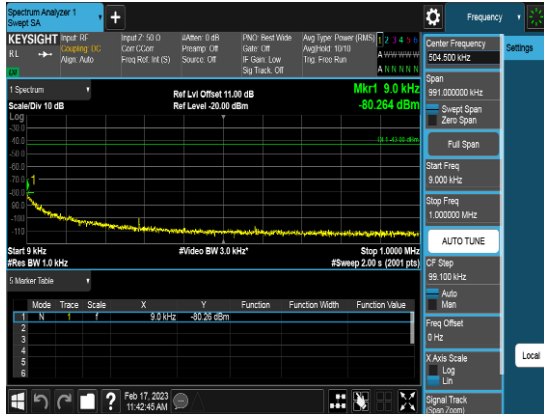
Port2_10M_3694.98MHz_TM3.1_CHH_CSE1
