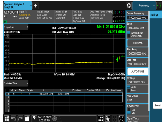
Port2_20M_3560.01MHz_TM3.1_CHL_CSEpart 6
