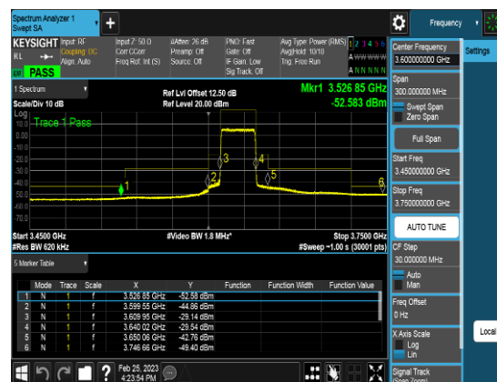
Port2_30M_3624.99MHz_TM3.1_CHM_CSEpart 96
