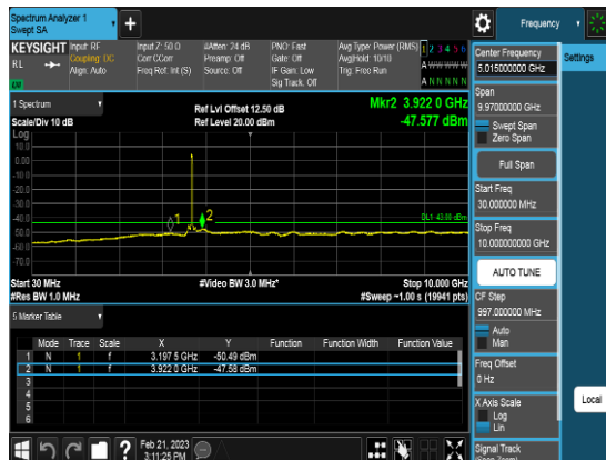
Port2_40M_3679.98MHz_TM3.1_CHH_CSE3
