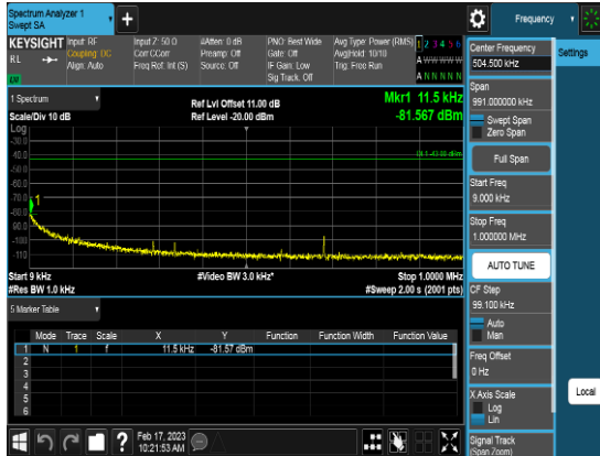
Port2_10M_3624.99MHz_TM3.1_CHM_CSE1
