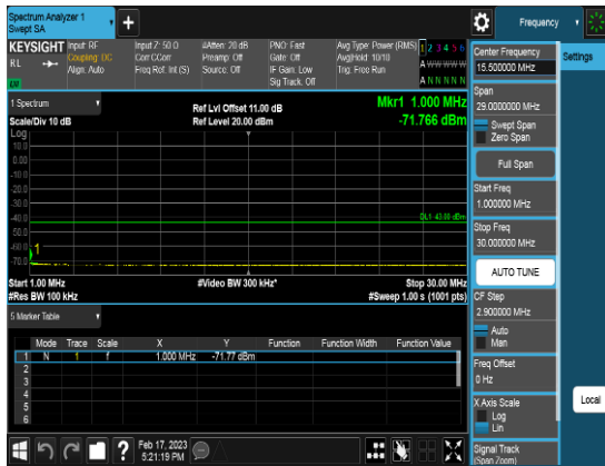
Port2_20M_3624.99MHz_TM1.1_CHM_CSE2
