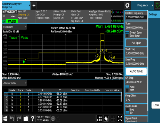
Port2_20M_3560.01MHz_TM1.1_CHL_CSE0b
