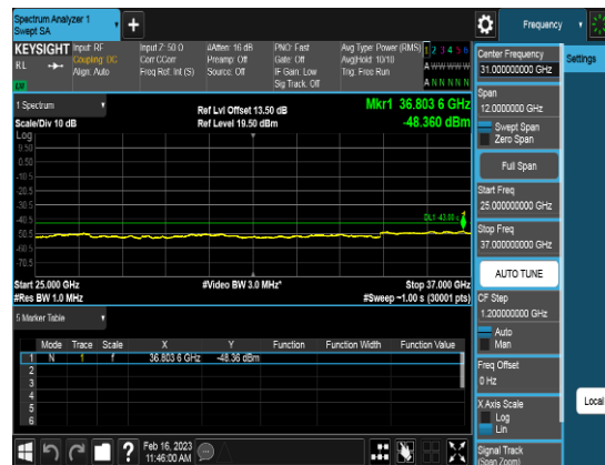
Port2_10M_3555MHz_TM1.1_CHL_CSE3
