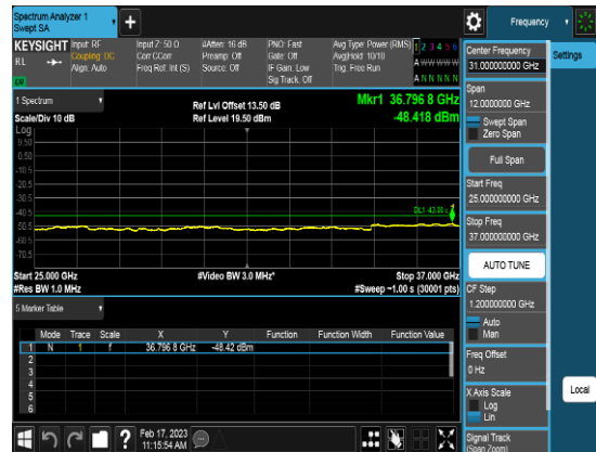
Port2_10M_3694.98MHz_TM1.1_CHH_CSE3
