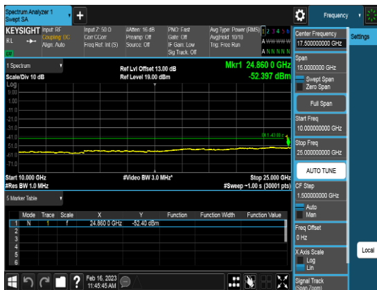
Port2_10M_3555MHz_TM1.1_CHL_CSE2
