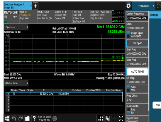
Port2_20M_3624.99MHz_TM1.1_CHM_CSE3
