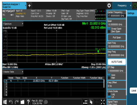
Port2_40M_3570MHz_TM1.1_CHL_CSE2
