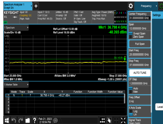
Port2_40M_3679.98MHz_TM1.1_CHH_CSE3
