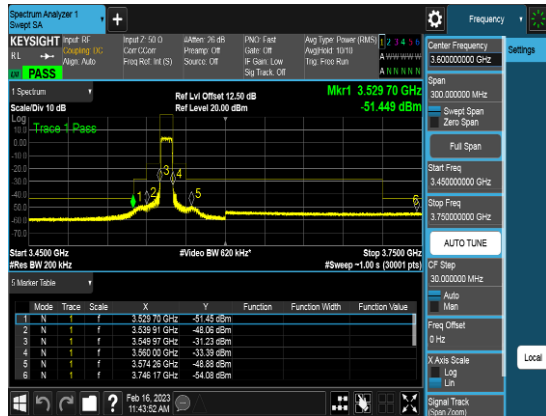
Port2_10M_3624.99MHz_TM1.1_CHM_CSE0b
