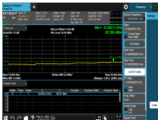
Port2_40M_3624.99MHz_TM1.1_CHM_CSE2
