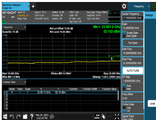
Port2_30M_3624.99MHz_TM1.1_CHM_CSE2
