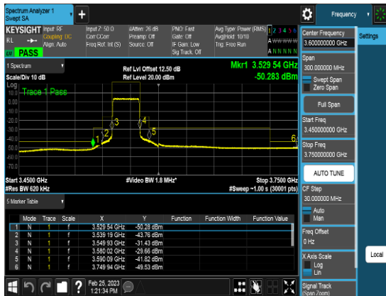
Port2_30M_3624.99MHz_TM1.1_CHM_CSE0b
