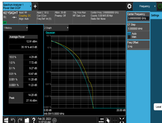
Port1_20M_3690MHz_TM3.1_CHH_PAPR
