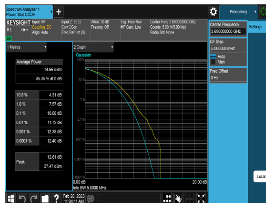
Port2_20M_3690MHz_TM1.1_CHH_PAPR
