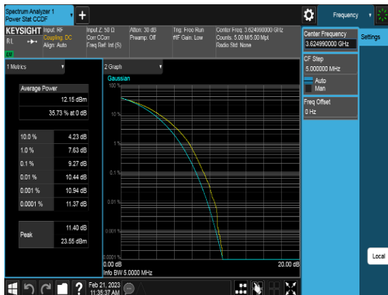
Port2_40M_3624.99MHz_TM3.1_CHM_PAPR
