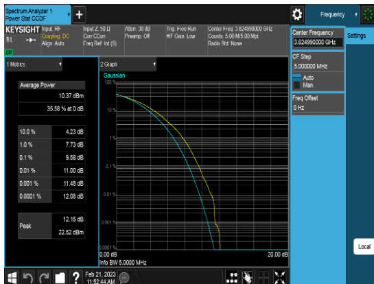
Port1_40M_3624.99MHz_TM3.1a_CHM_PAPR
