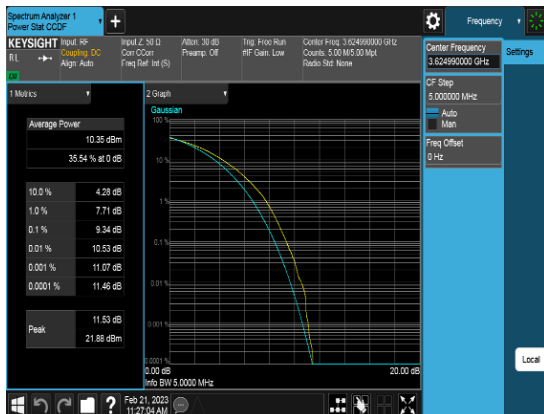
Port1_40M_3624.99MHz_TM3.1_CHM_PAPR
