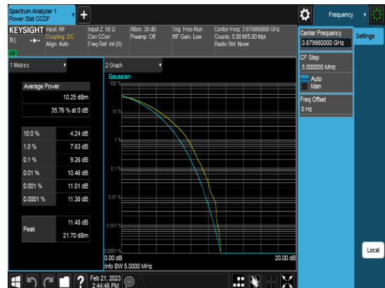
Port1_40M_3679.98MHz_TM3.1_CHH_PAPR
