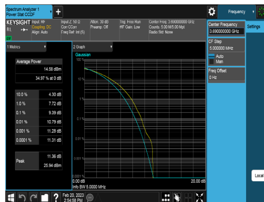
Port2_20M_3690MHz_TM3.1a_CHH_PAPR
