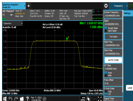
Port2_20M_3624.99MHz_TM1.1_CHM_PSD
