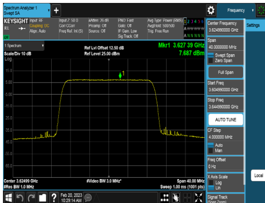
Port2_20M_3624.99MHz_TM3.1a_CHM_PSD
