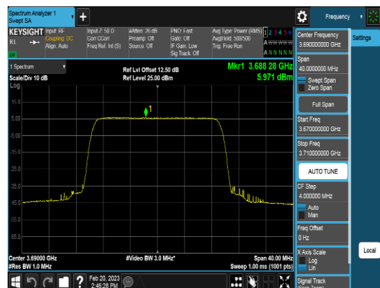
Port1_20M_3690MHz_TM3.1a_CHH_PSD
