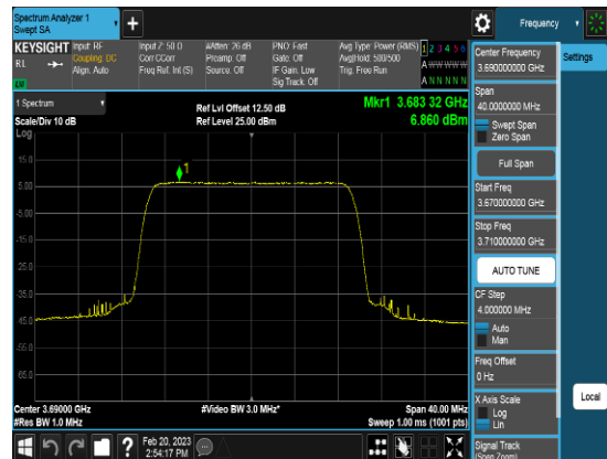
Port2_20M_3690MHz_TM3.1a_CHH_PSD
