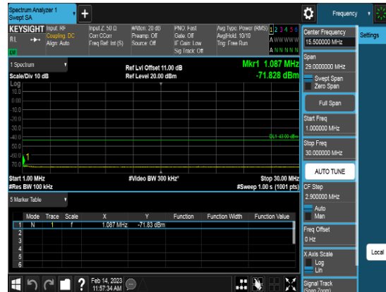
Port1_10M_3625MHz_TM3.2_CHM_CSE2
