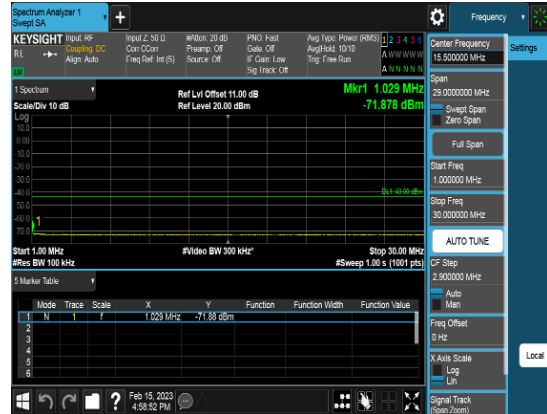
Port1_20M_3690MHz_TM3.2_CHH_CSE2
