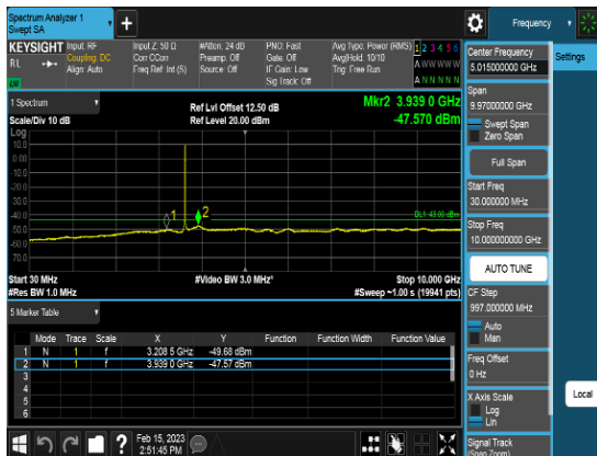
Port2_20M_3625MHz_TM3.2_CHM_CSE3
