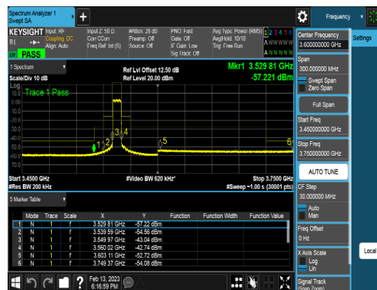
Port1_10M_3555MHz_TM3.1_CHL_CSEpart96
