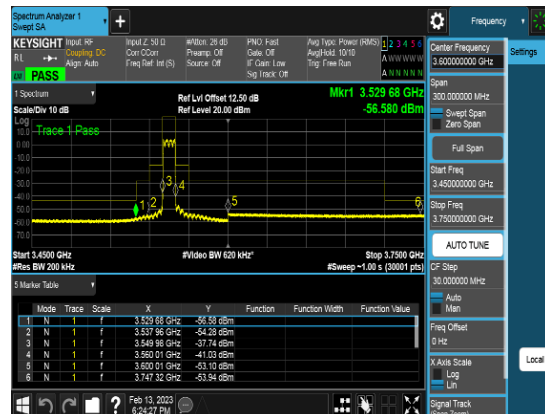
Port2_10M_3555MHz_TM3.1_CHL_CSEpart96
