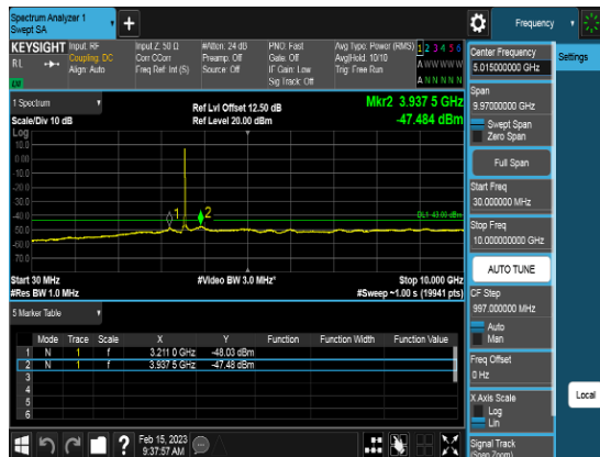
Port1_20M_3560MHz_TM3.1_CHL_CSE3
