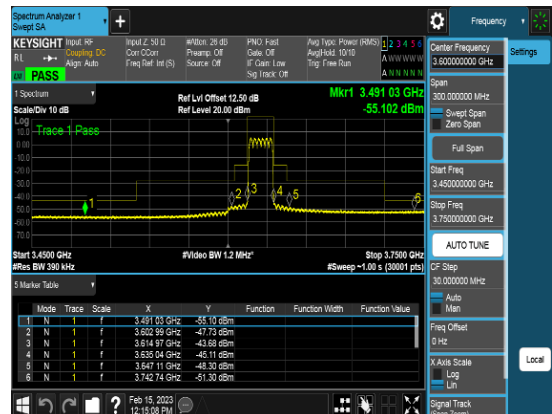
Port1_20M_3625MHz_TM3.1_CHM_CSEpart96
