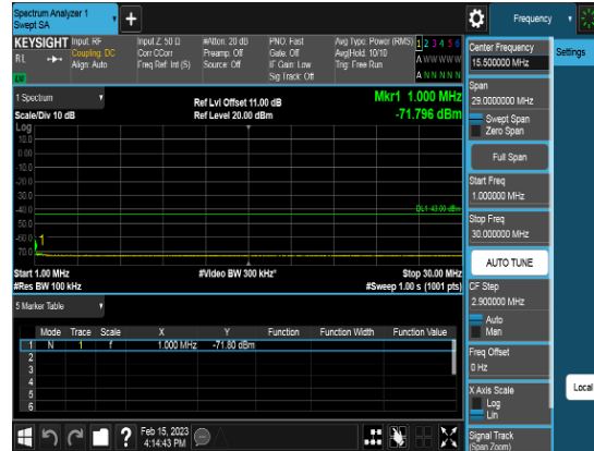
Port1_20M_3690MHz_TM3.1_CHH_CSE2
