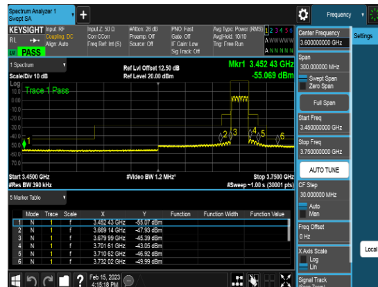
Port1_20M_3690MHz_TM3.1_CHH_CSEpart96
