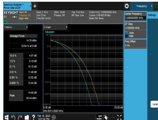
Port2_20M_3690MHz_TM3.2_CHH_PAPR
