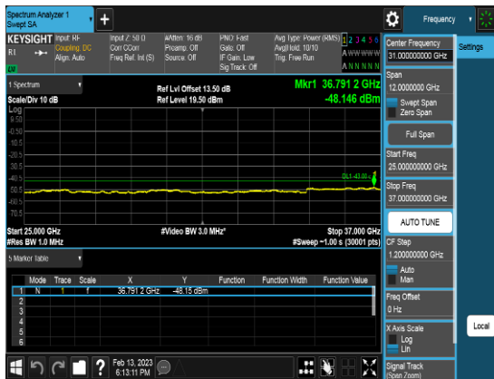
Port1_10M_3555MHz_TM3.1_CHL_CSE3
