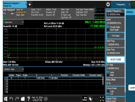
Port2_20M_3625MHz_TM3.1_CHM_CSE2
