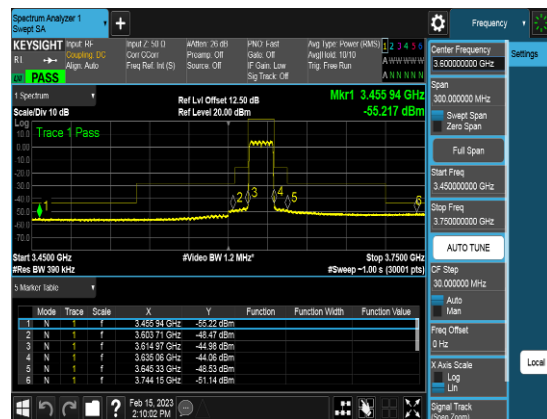
Port2_20M_3625MHz_TM3.1_CHM_CSEpart96
