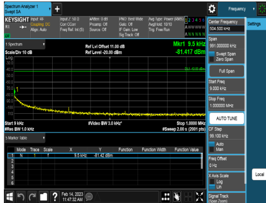
Port1_10M_3625MHz_TM3.1_CHM_CSE1
