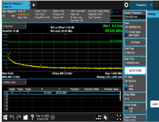
Port1_10M_3555MHz_TM3.1_CHL_CSE1
