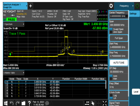
Port2_10M_3625MHz_TM3.1_CHM_CSEpart96
