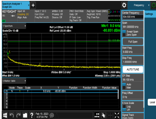
Port2_20M_3690MHz_TM3.1_CHH_CSE1
