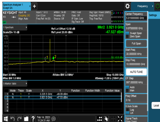
Port1_10M_3625MHz_TM3.1_CHM_CSE3
