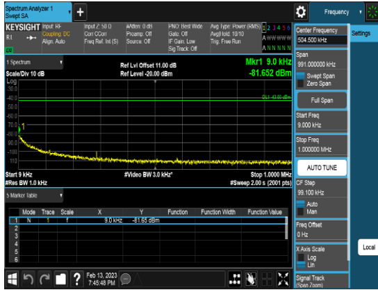
Port1_10M_3555MHz_TM3.2_CHL_CSE1
