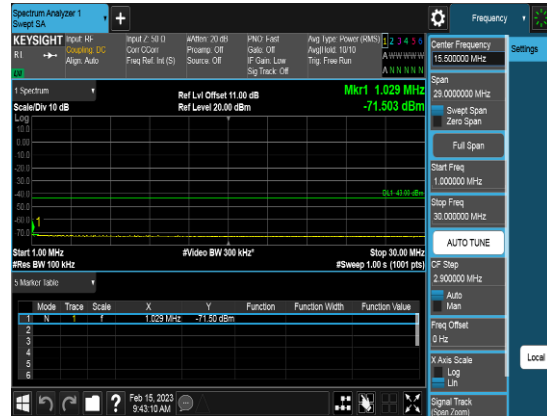
Port1_20M_3560MHz_TM3.1_CHL_CSE2
