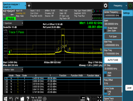
Port1_10M_3625MHz_TM3.1_CHM_CSEpart96
