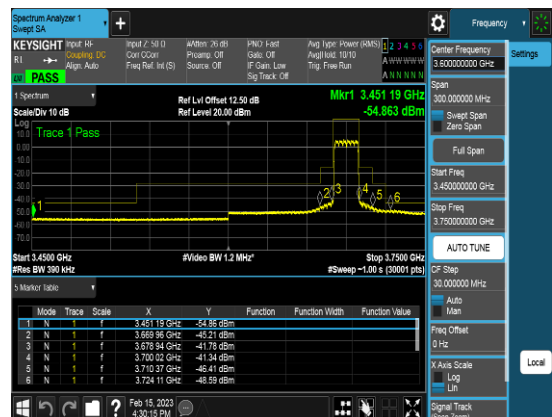
Port2_20M_3690MHz_TM3.1_CHH_CSEpart96
