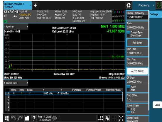
Port2_10M_3625MHz_TM3.1_CHM_CSE2
