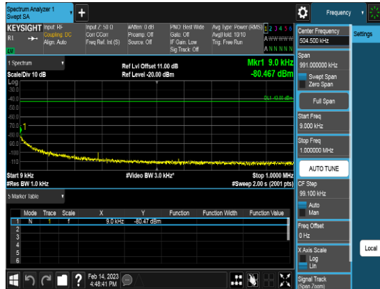
Port2_10M_3695MHz_TM3.1_CHH_CSE1
