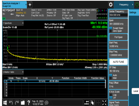
Port1_20M_3560MHz_TM3.1_CHL_CSE1
