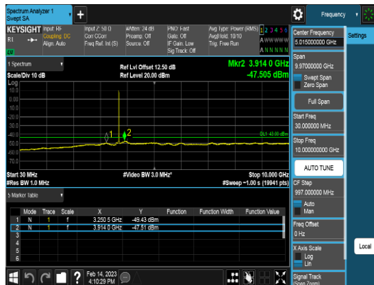
Port1_10M_3695MHz_TM3.1_CHH_CSE3
