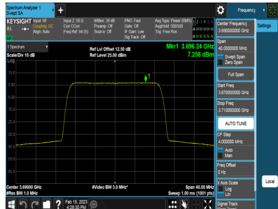
Port2_20M_3690MHz_TM3.1_CHH_PSD
