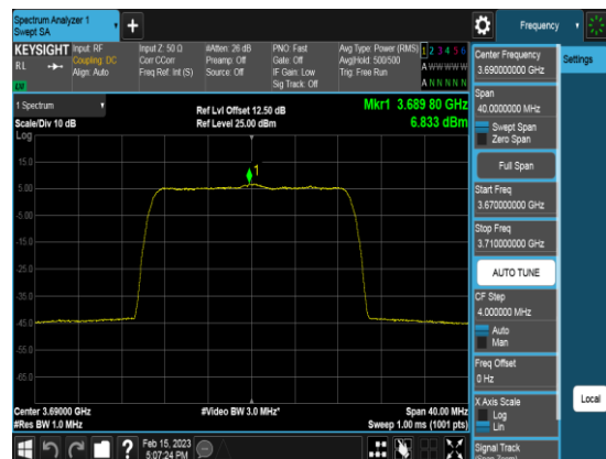
Port1_20M_3690MHz_TM3.2_CHH_PSD
