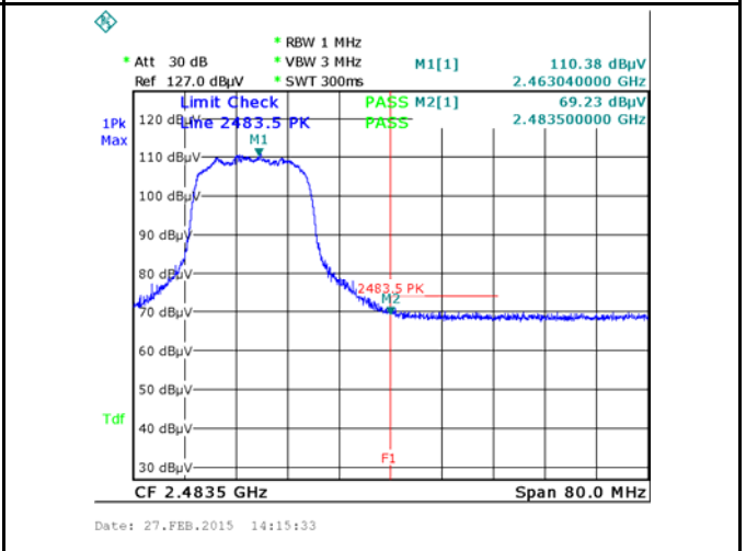
Band Edge, Right Side (Peak) - 802.11n(20M) (EMW3165-E)
