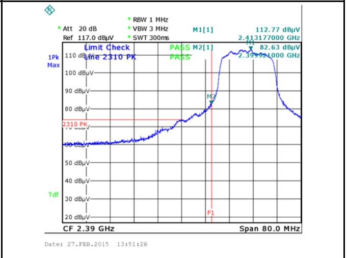
Band Edge, Left Side (Peak) - 802.11n(20M) (EMW3165-E)
