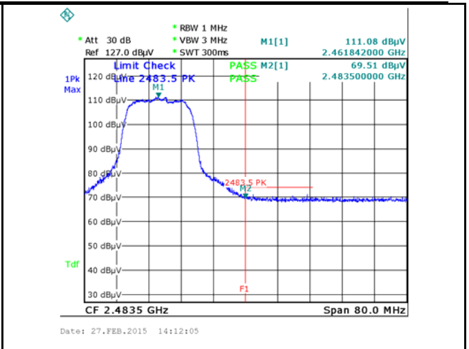
Band Edge, Right Side (Peak) - 802.11g (EMW3165-E)
