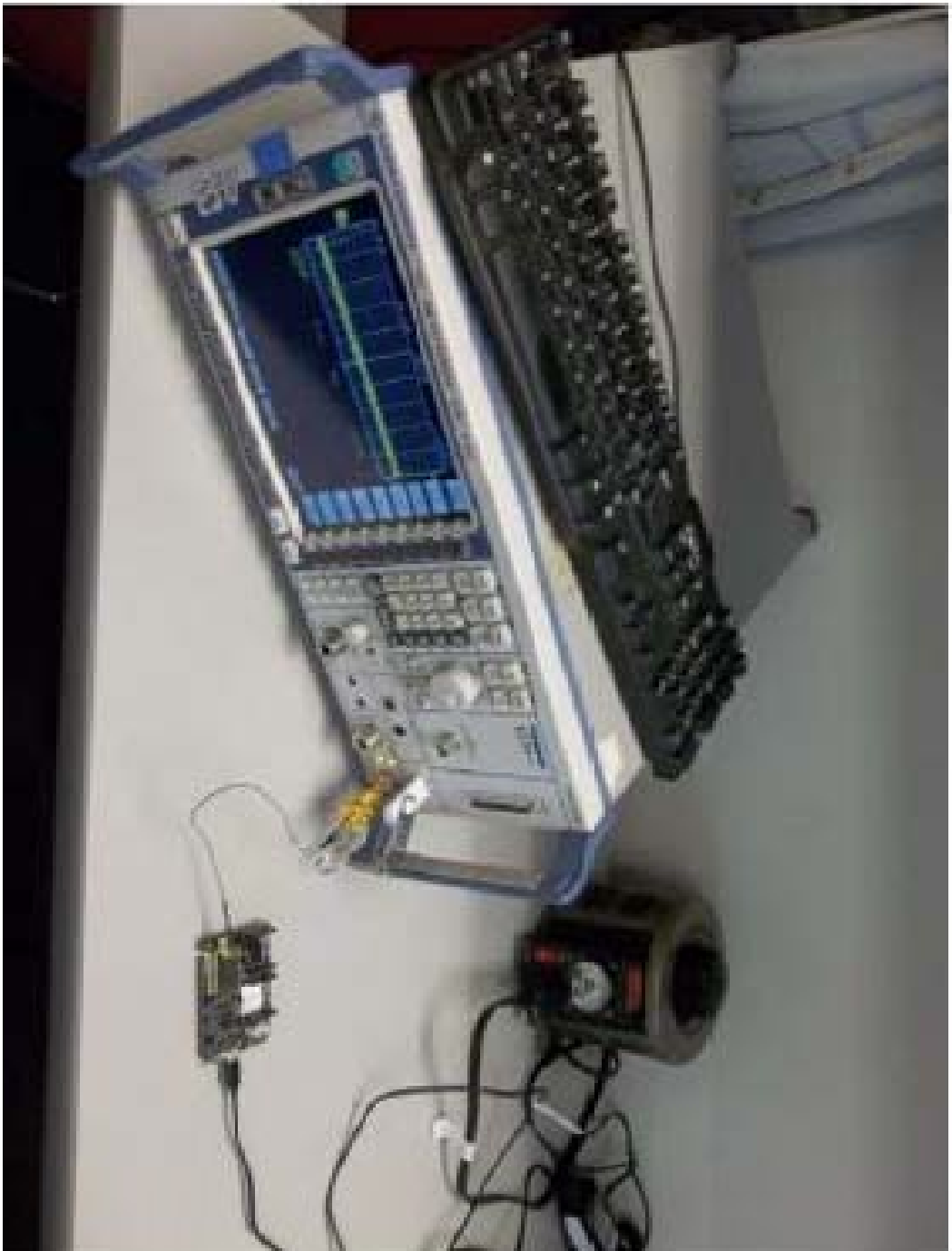
General Conducted Test Setup
