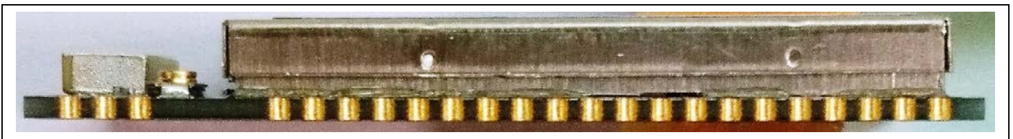
Lower Edge – Chip Antenna & RF Connector at Left of Picture
