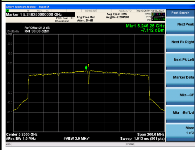
Channel 50 (5250MHz)
