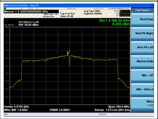
Channel 114 (5570MHz)
