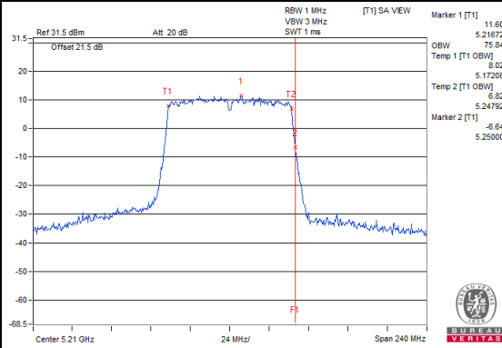
802.11ac(VHT80)_Chain0 / CH42
