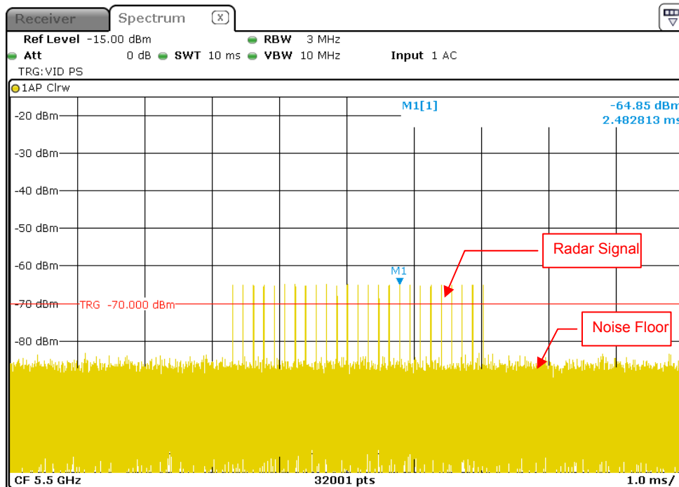
Radar Signal 2
