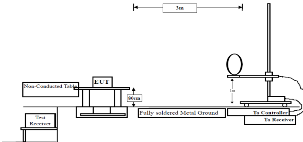
Figure 1. Below 30MHz
