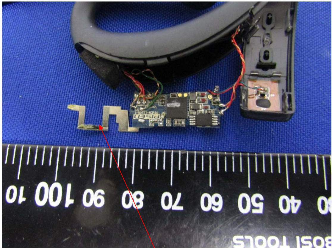
BT Antenna
