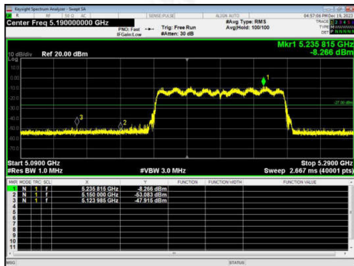
(802.11ac80) Band Edge, Left Side
