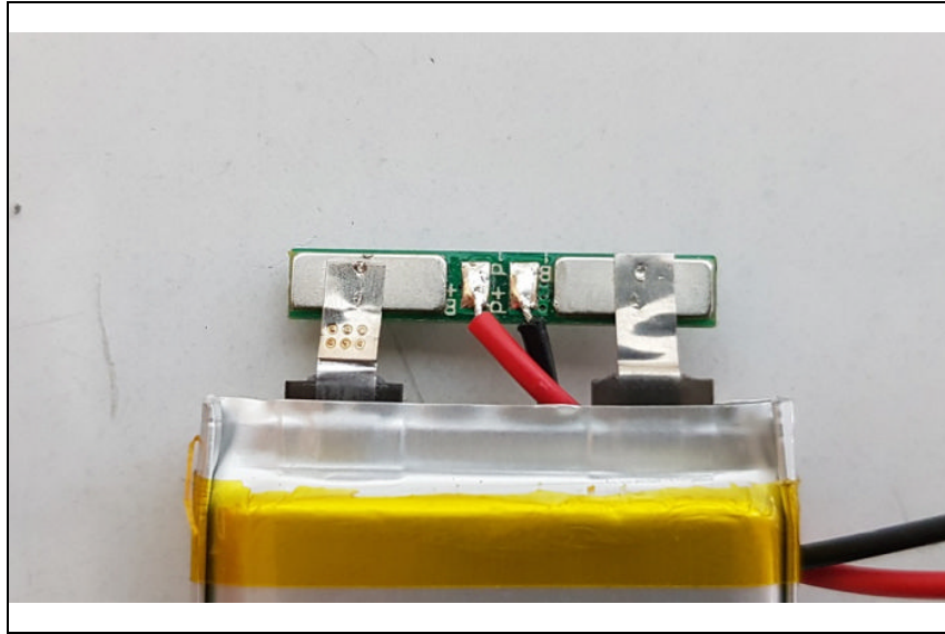
Top view of Sub4 PCB
