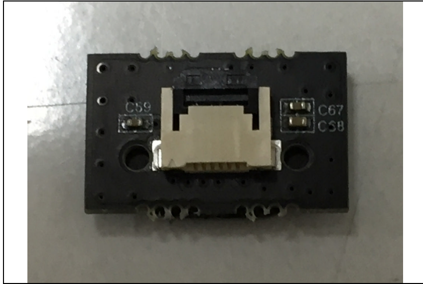
Top view of Sub2 PCB
