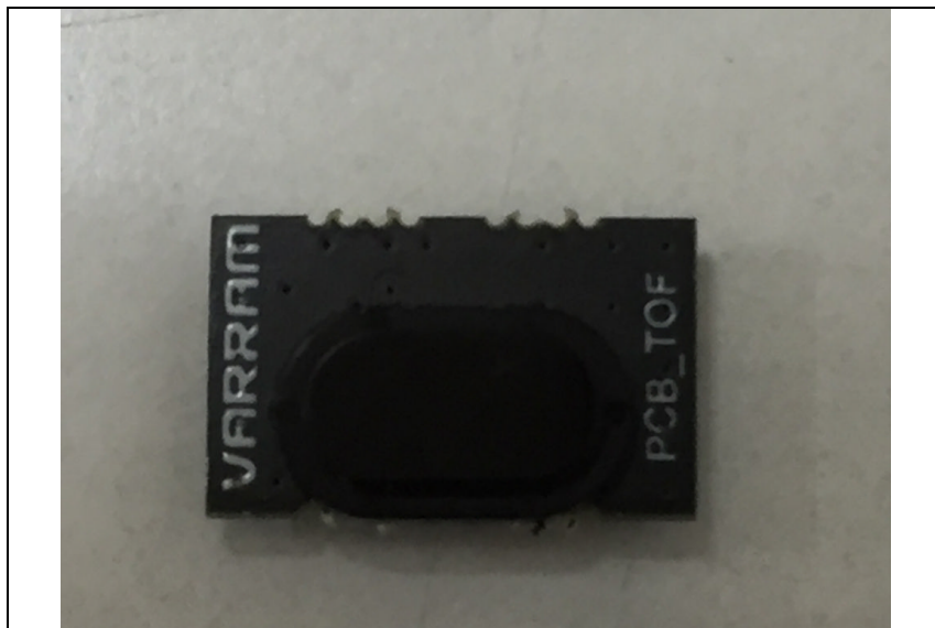
Bottom view of Sub2 PCB
