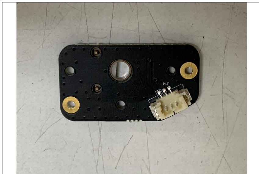
Bottom view of Sub4 PCB
