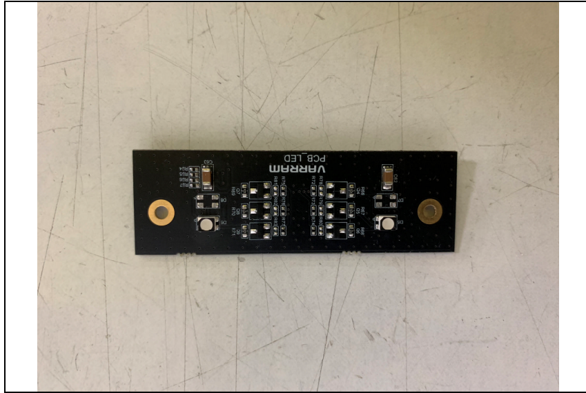
Top view of Sub1 PCB
