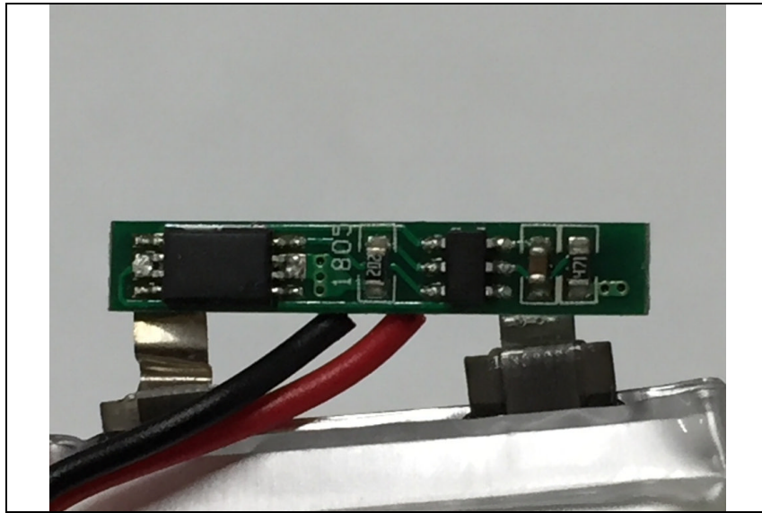
Top view of Sub3 PCB
