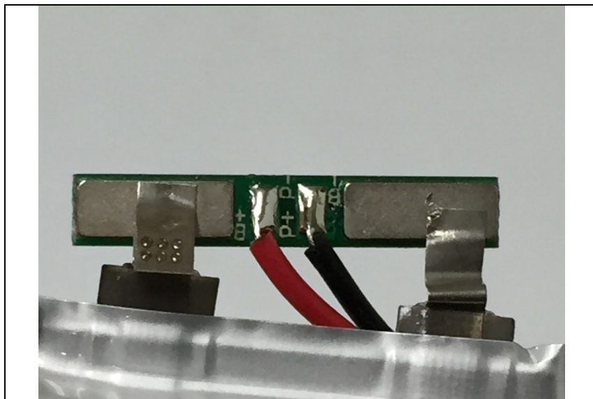
Bottom view of Sub3 PCB
