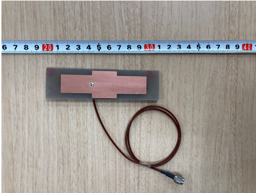
Antenna 2
