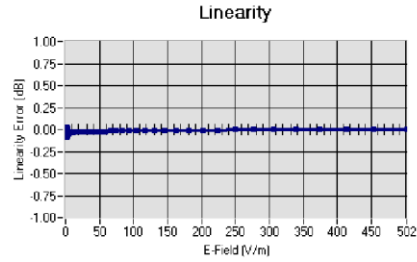
Linearity: \pm 1.91\% ( \pm 0.08\text{dB} )
