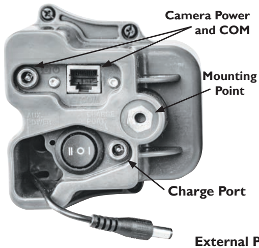
Transmitter (Photo 2)
