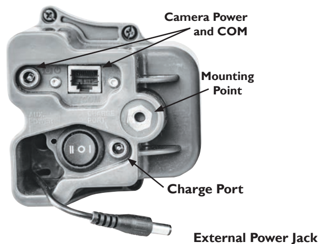
Transmitter (Photo 1)
