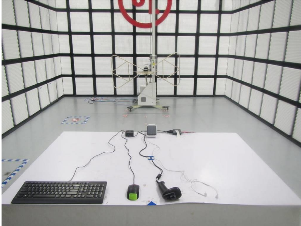
Radiated Emissions below 1GHz test setup photo
