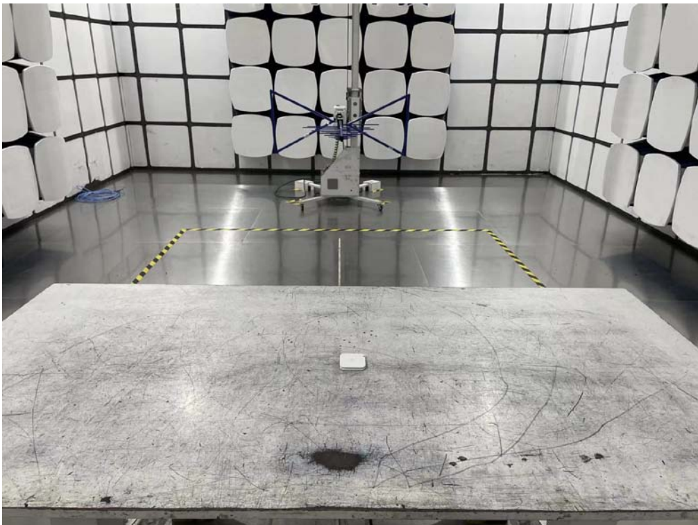
Radiated emission test: 30-1000MHz
