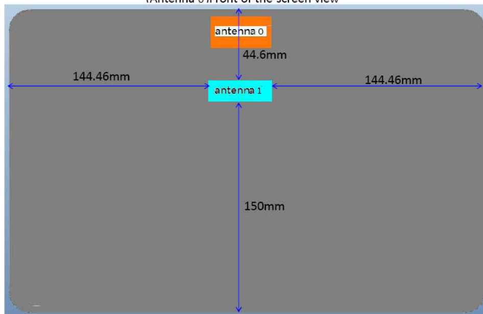
(Antenna 1)Front of the screen view
