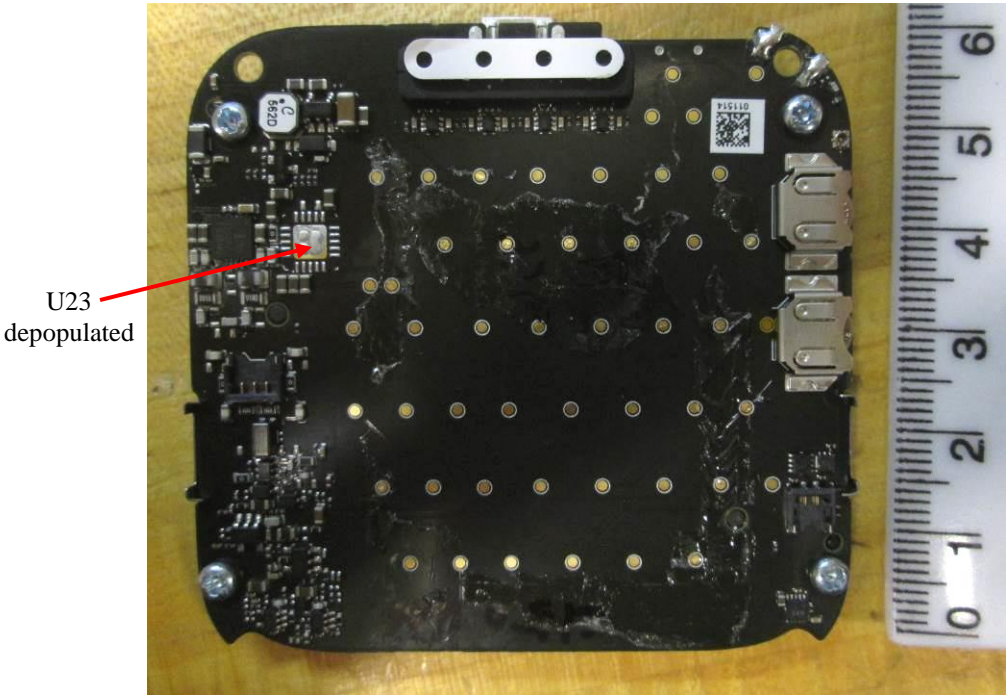
EUT after C2PC– Internal view 8 PCB, side 2, battery removed
