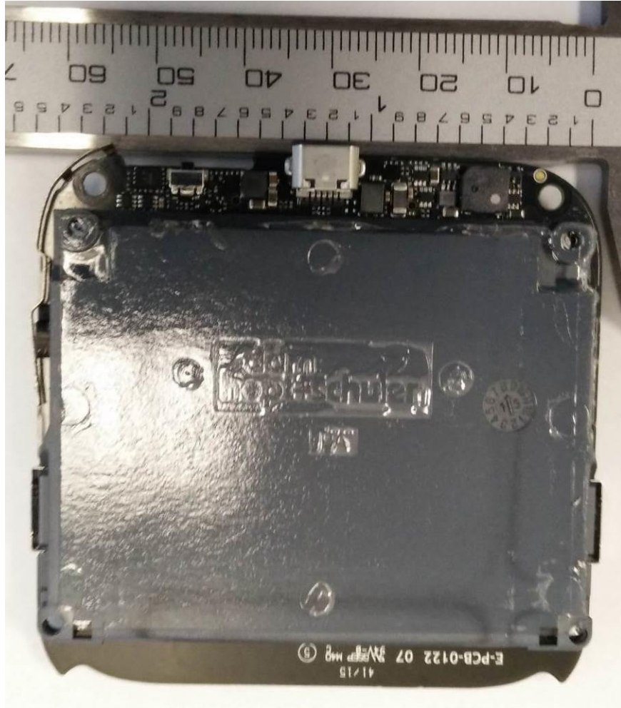
EUT – Internal view 2 PCB, side 1, with cage
