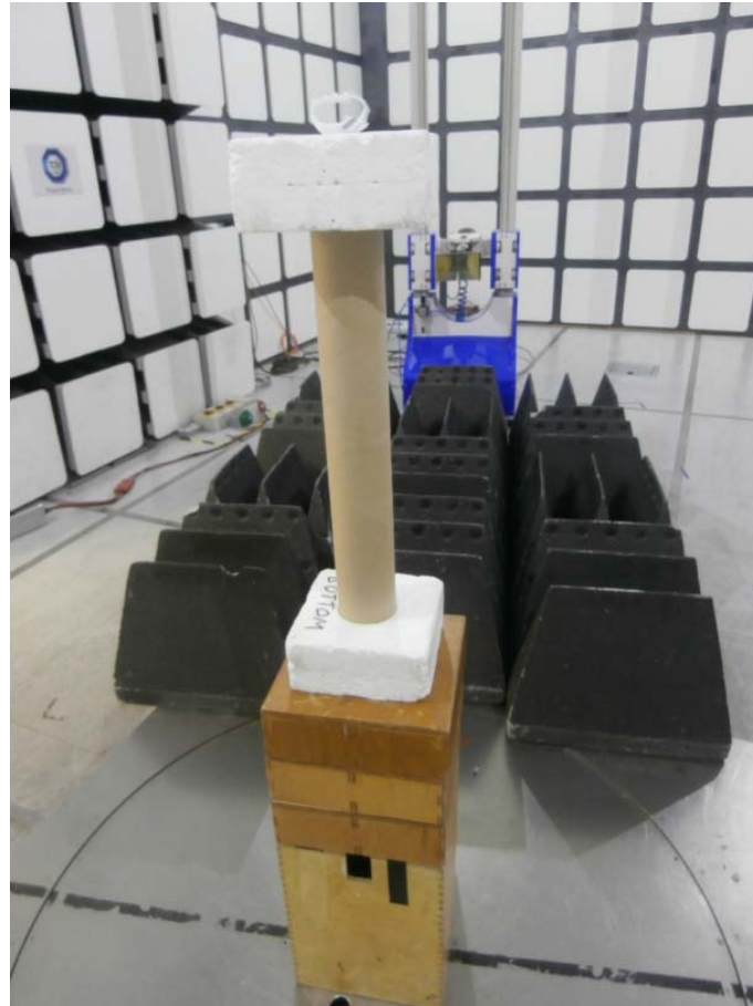
FCC 15C Radiated Emissions 1 GHz to 18 GHz
