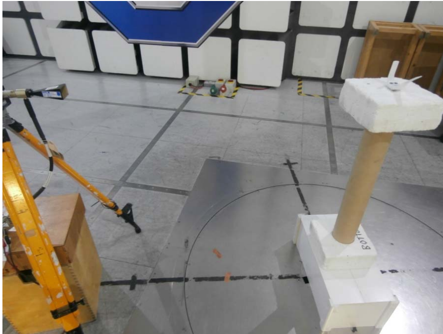
FCC 15C Radiated Emissions 18 GHz to 25 GHz
