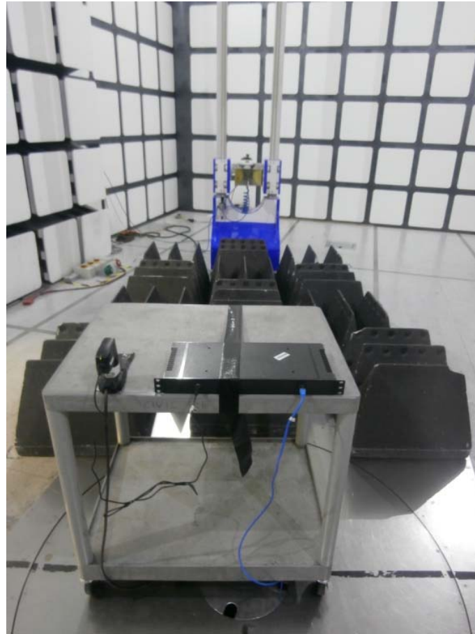
FCC 15B Radiated Emissions 1 GHz to 13 GHz
