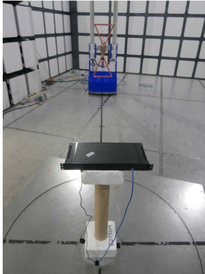
FCC 15C Radiated Emissions 30 MHz to 1 GHz
