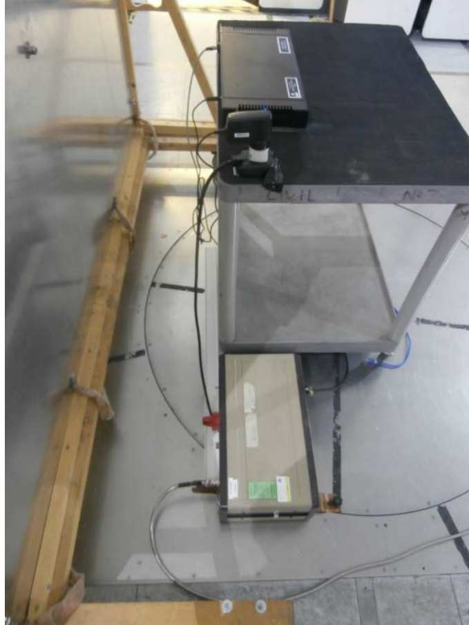
AC Line Conducted Emissions
